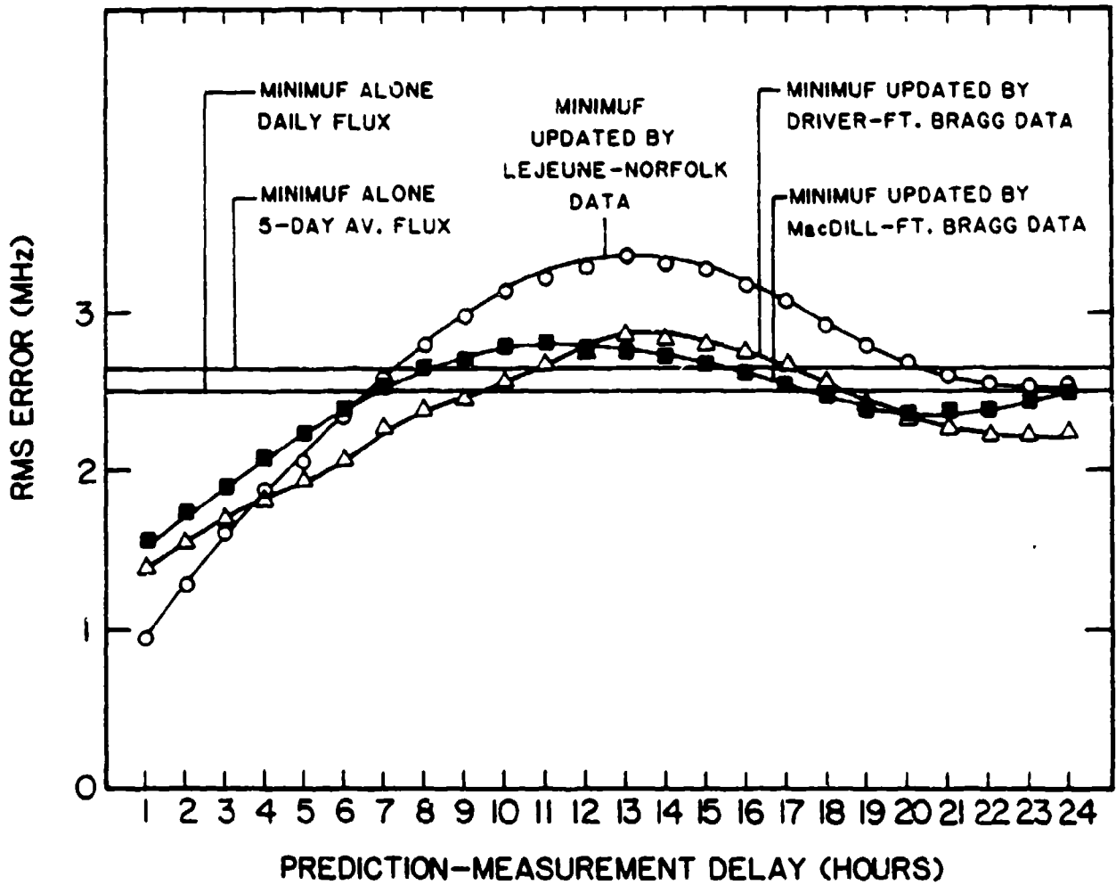
Fig. 8 - RMS error between actual MOFs on the Lejeune to Norfolk path and MOFs predicted by a variety of techniques, as a function of time delay between prediction and measurement. Data include approximately 335 hourly predictions for each value of time delay.
