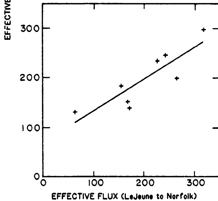
Fig. 3 — Effect of removing "wild points" from the correlation data. Both plots show the correlation of effective fluxes on the MacDill-Norfolk, LeJeune-Norfolk paths for the hour 1500-1600Z. In the lower plot, two "wild points" have been subjectively removed. Straight lines are least-squares regression fits to the data.
