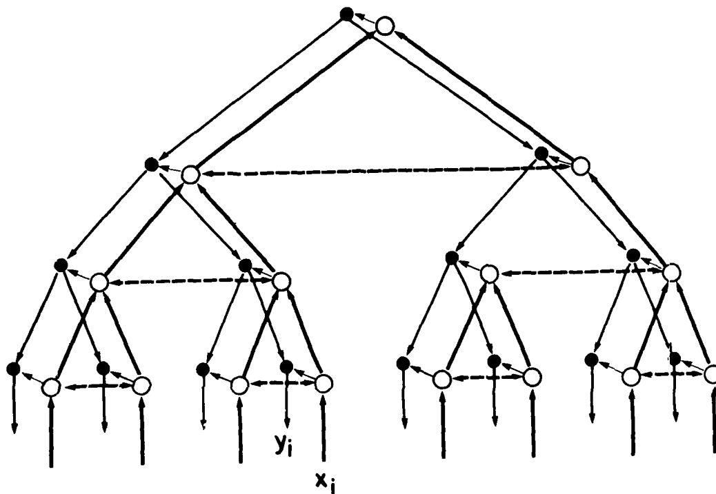
Figure 3. A possible implementation of the Winner-Take-All network with n = 8 input units. The local comparison takes place between m = 2 units. The more active unit inhibits the less active one and excites the unit on the next level. The auxiliary units, drawn in black, are only activated if they receive conjointly excitation from their associated main unit and from the auxiliary unit at the higher level. The auxiliary unit y_i , corresponding to the most active unit x_i in the saliency map, will be activated after at most 2\log_2 n = 8 time steps. In order to insure stability against noise and to enforce neighborhood relations between all neighboring points (for instance between the two middle units, belonging to two different subtrees) additional connections (and units) can be added between (and within) levels. We have just shown the most sparse implementation of a WTA network.
