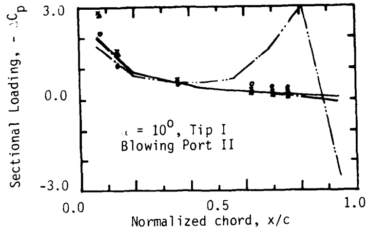
Figure 36. Comparison of Theory vs Measurements on Chordwise Sectional Loading
