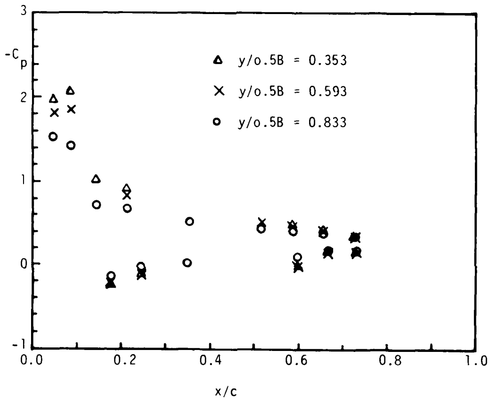
Figure 5. Pressure distribution on the wing for \alpha = 10^\circ , no blowing.
