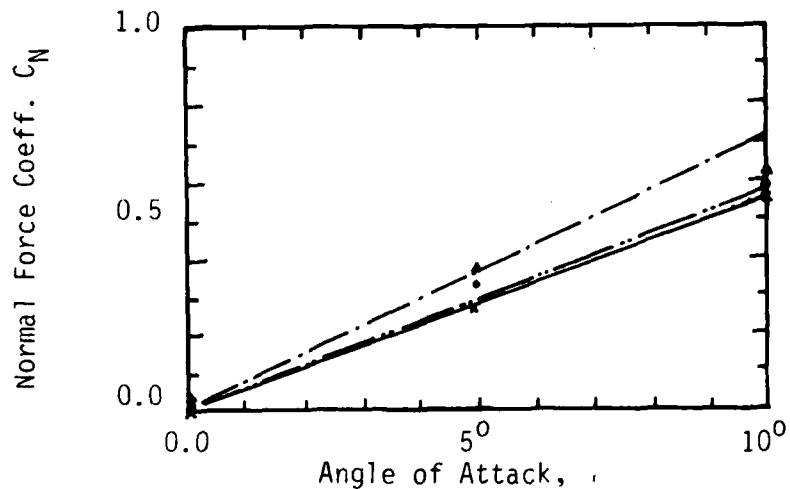
Figure 37. Comparison of Theory and Experiments on Integrated Normal Force Coefficient
