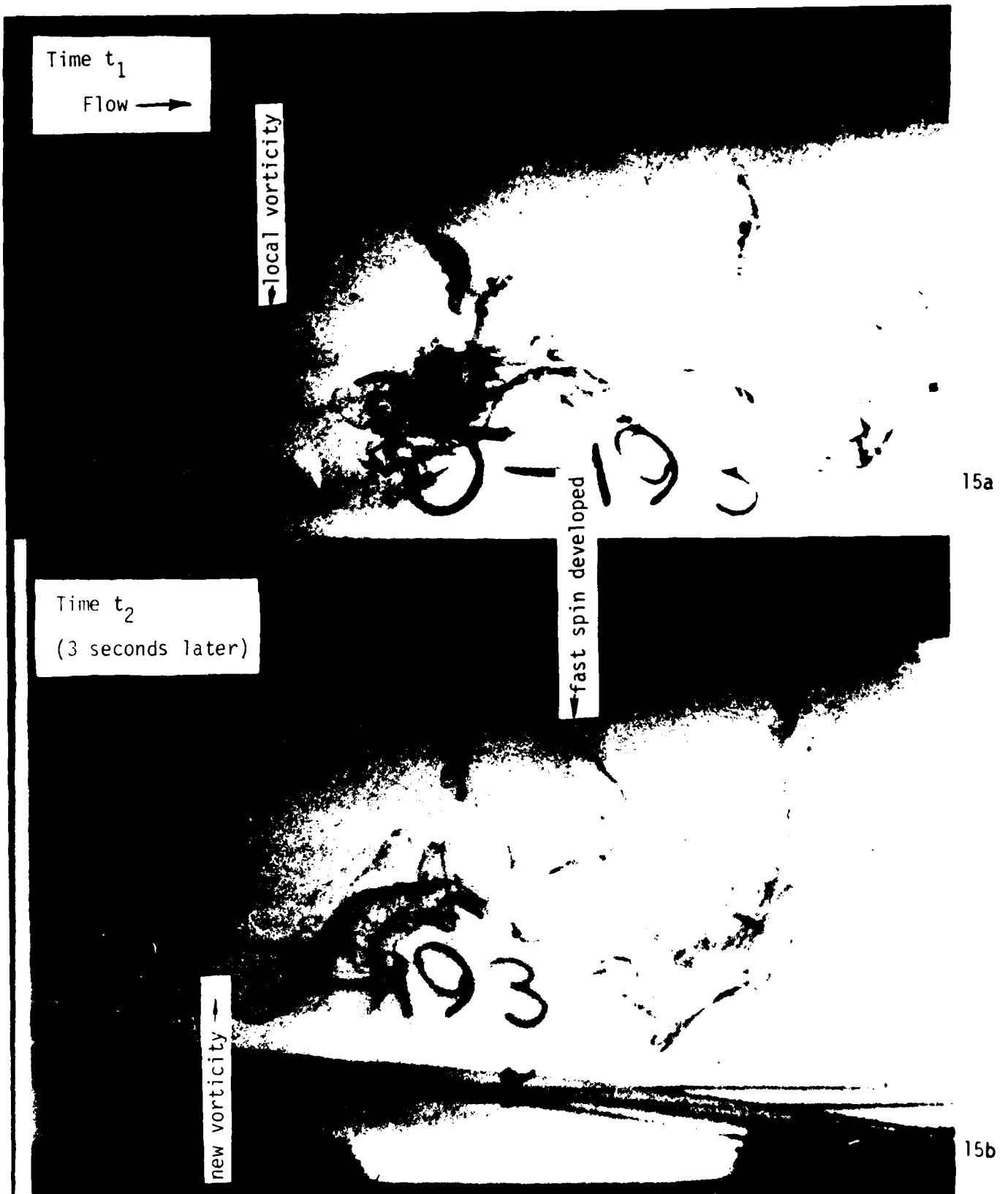
Figure 15. Time Sequence of Development of Secondary "Spin-Off" Vortices.
