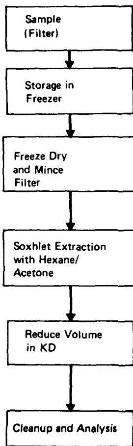
Figure 26. Flow Scheme of the Extraction Procedure for Filtered Suspended Sediments
