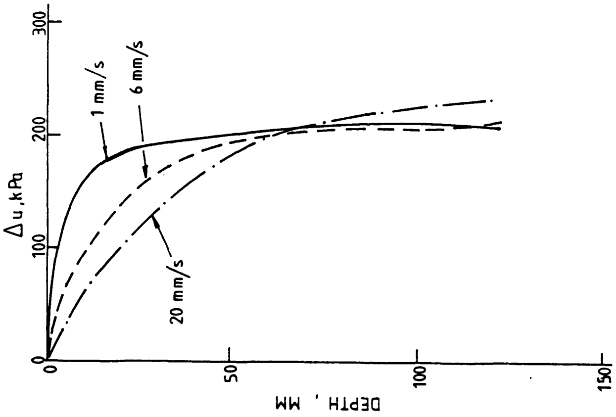
Fig. 5.9: Influence of the rate of penetration in Gault clay, OCR = 10
