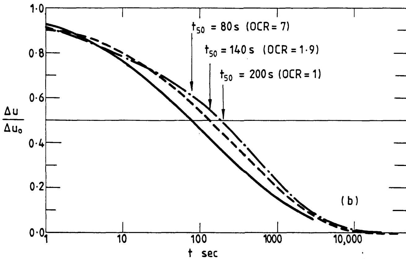
Fig. 5.12. Dissipation curves for different OCR values.
