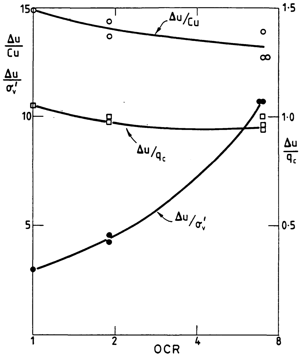
Fig. 5.11: Variation of the normalized pore pressure with OCR for Gault clay
