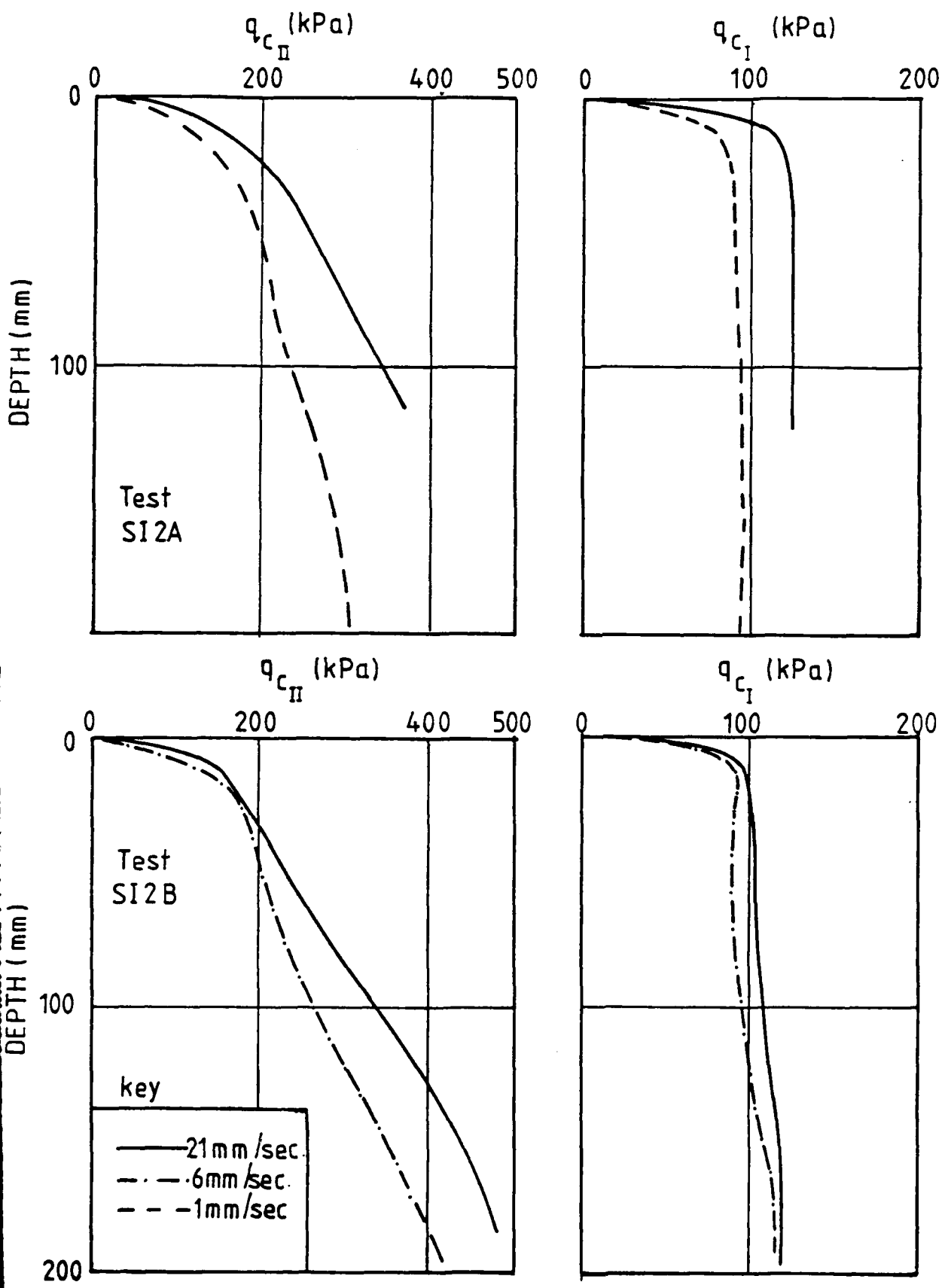
Fig. 4.7: Cone penetrometer tests with Mark II probe
