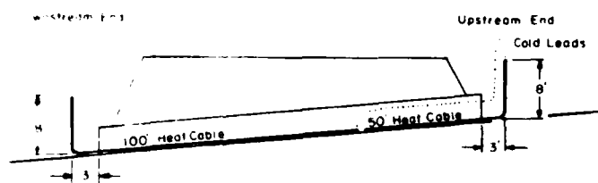
a. Culvert profile showing cable installation.
