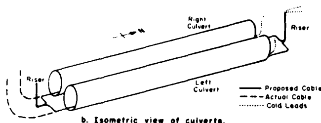
b. Isometric view of culverts.
