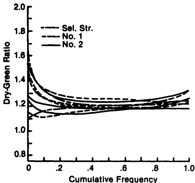
Figure 7.—Effect of position in the MOE distribution on the dry-green ratio of lumber dried to 15 percent moisture content (ratios obtained from fitted three-parameter Weibull distribution). (ML84 5262)
