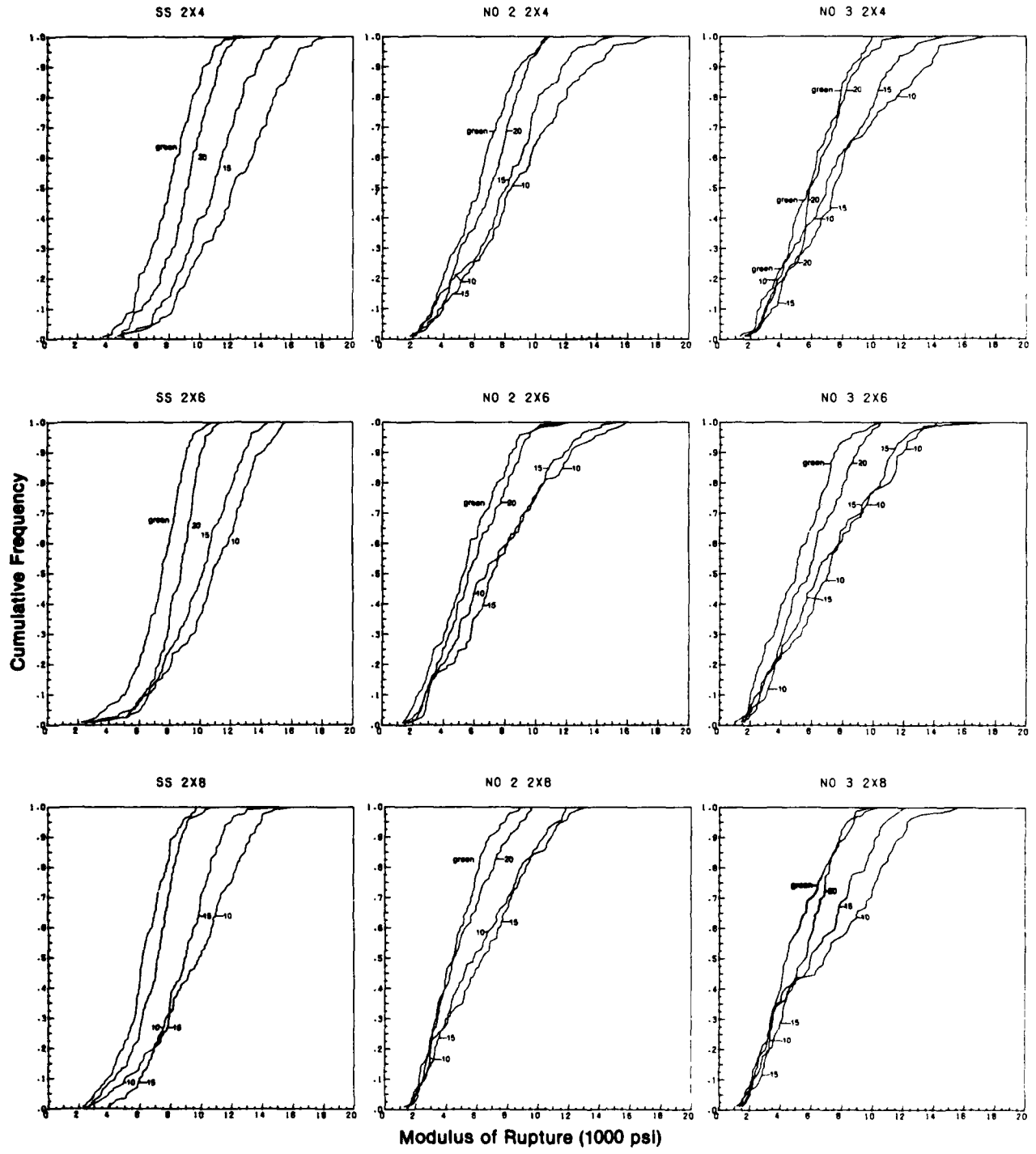
Figure B1.—Cumulative frequency distributions for MOR at the four moisture content levels. (ML84 5268)
