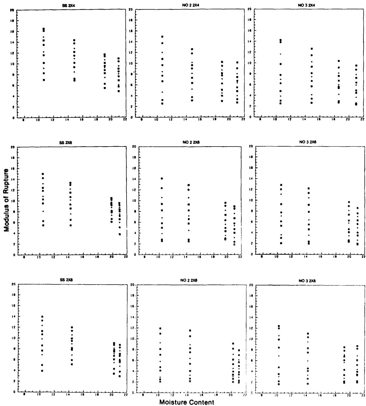
Figure B5.—Effect of moisture content on modulus of rupture ( 10^3 psi) at various percentile levels (5, 10, 20...80, 90, 95). Percentiles plotted at average moisture content for the groups (21 pct for green). (ML84 5270)
