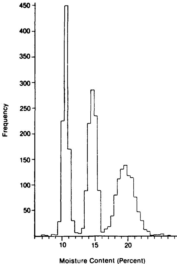
Figure 2.—Distribution of the moisture content of lumber after conditioning to target moisture contents of 10, 15, and 20 percent. (ML84 5318)
