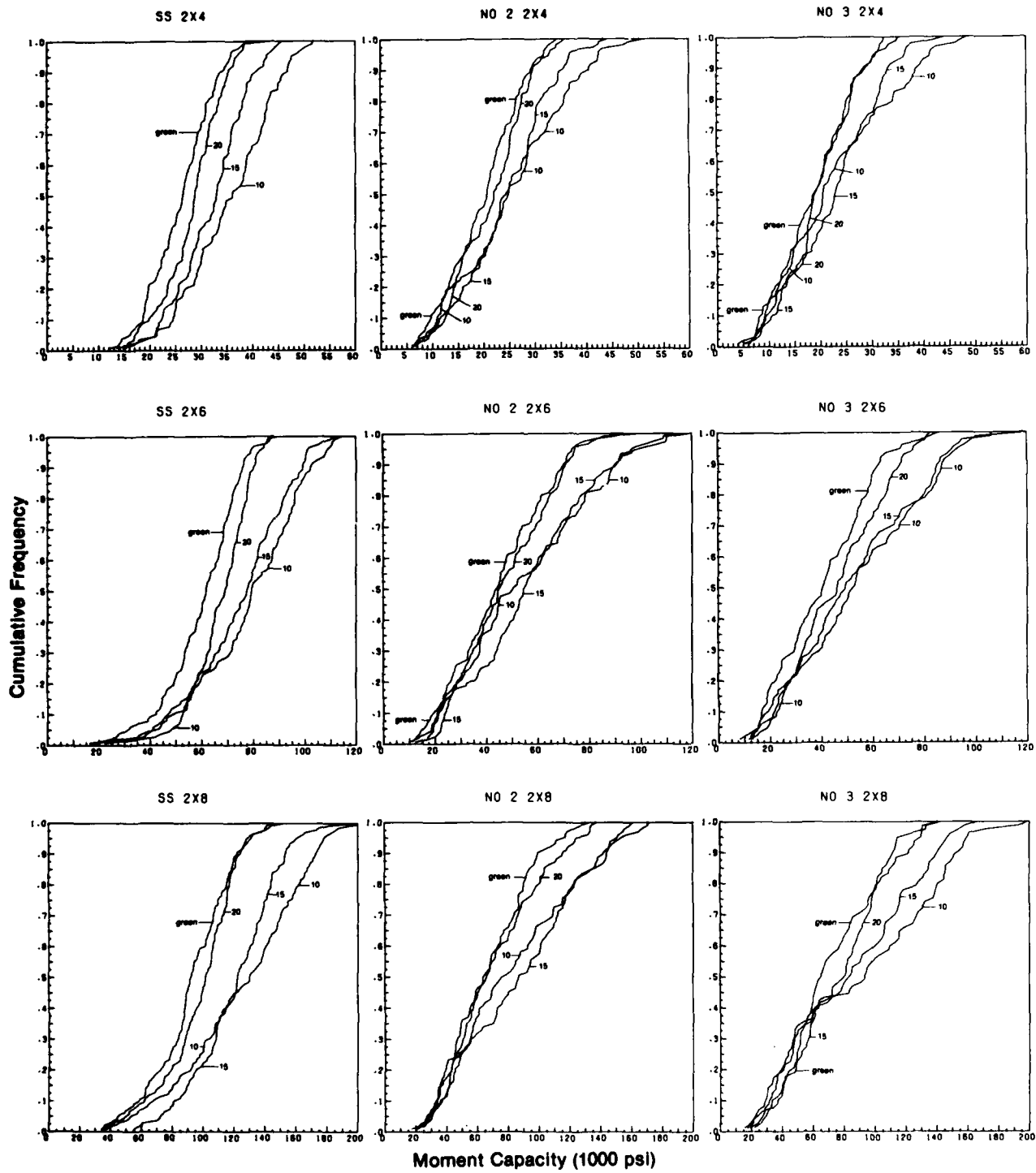
Figure B3.—Cumulative frequency distribution for RS at four moisture content levels. (ML84 5206)
