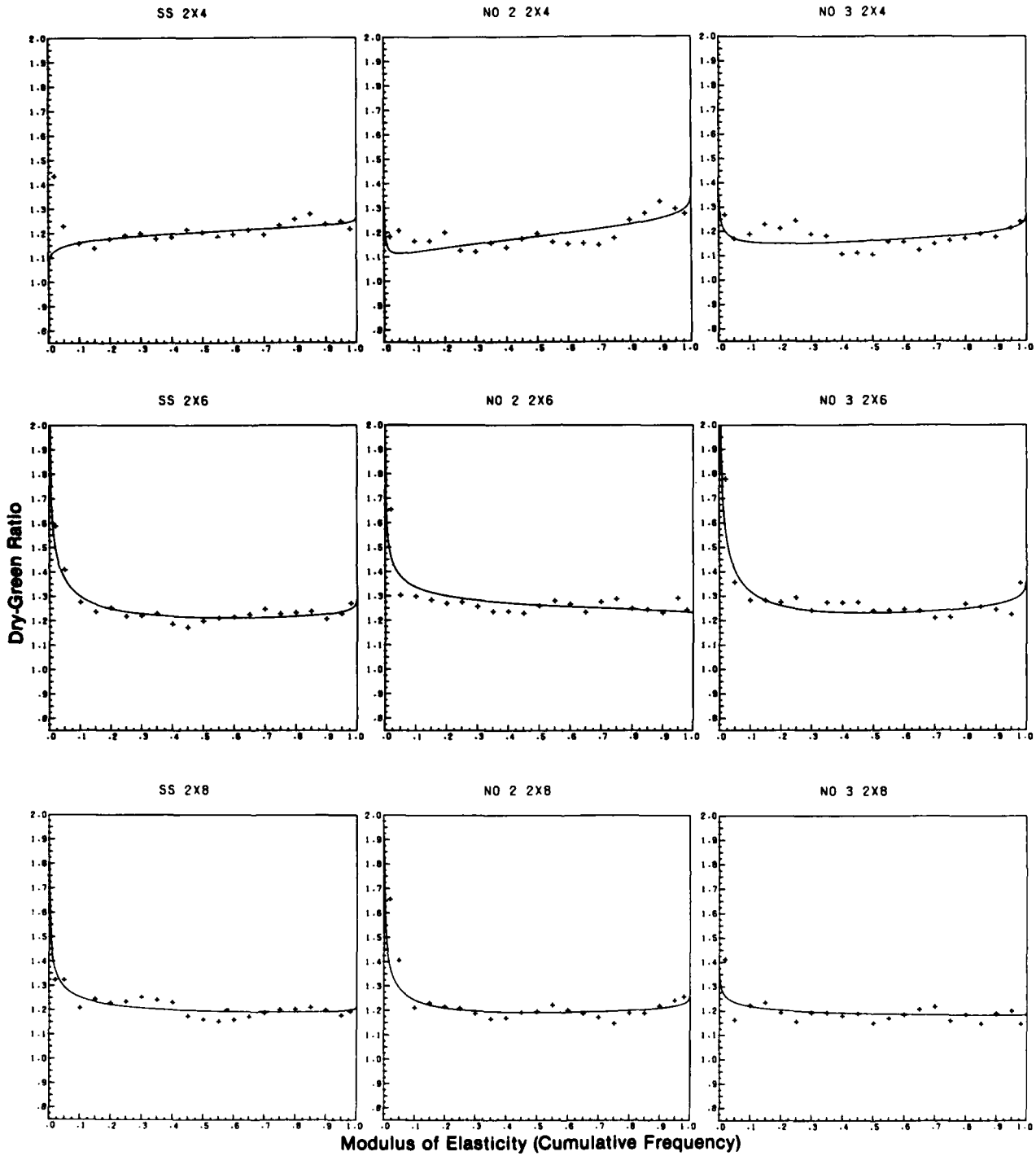
Figure B8.—Effect of percentile level on the modulus of elasticity dry-green ratio for lumber dried to a moisture content of 15 percent ("+" = experimental ratio at 2, 5, 10, 15... 90, 95, 98 percentiles; solid line = ratio obtained by first fitting three-parameter Weibull distributions to the MOE values ( 10^6 psi) for 15 percent and green moisture contents). (ML84 5269)
