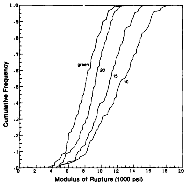
Figure 4.—Cumulative frequency distributions for MOR of 2 by 4 Select Structural lumber. (ML84 5320)
