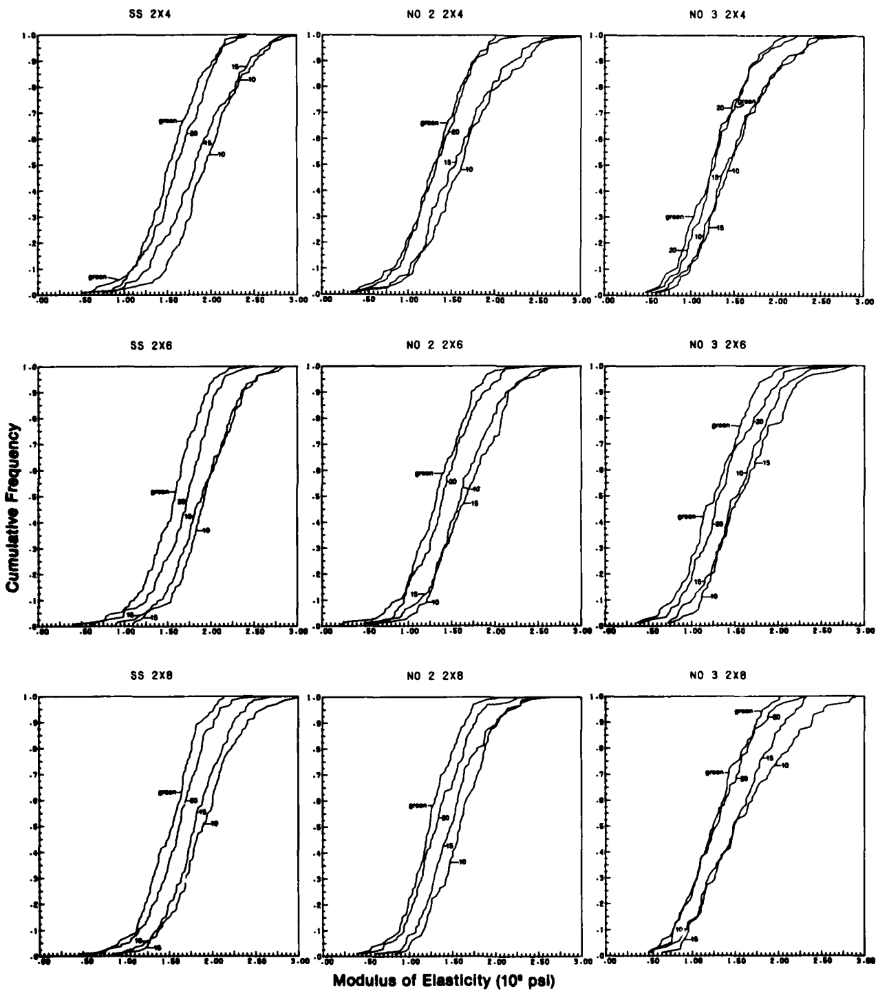
Figure B2.—Cumulative frequency distributions for MOE at the four moisture content levels. (MLB4 5267)
