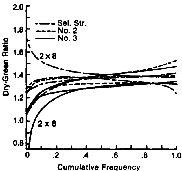
Figure 5.—Effect of position in the MOR distributions on the dry-green ratio of lumber dried to 15 percent moisture content (ratios obtained from fitted three-parameter Weibull distributions). (ML84 5261)
