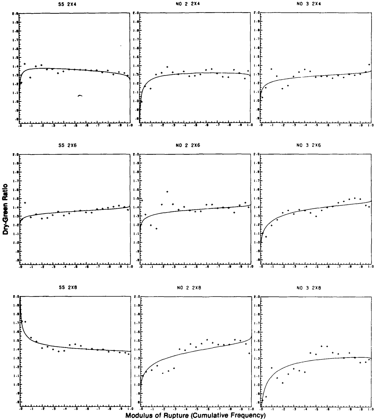
Figure B7.—Effect of percentile level on the modulus of rupture dry-green ratio for lumber dried to a moisture content of 15 percent ("+" = experimental ratio at 2, 5, 10, 15... 90, 95, 98 percentiles; solid line = ratio obtained by first fitting three-parameter Weibull distributions to the MOR values ( 10^3 psi) for 15 percent and green moisture contents). (ML84 5265)
