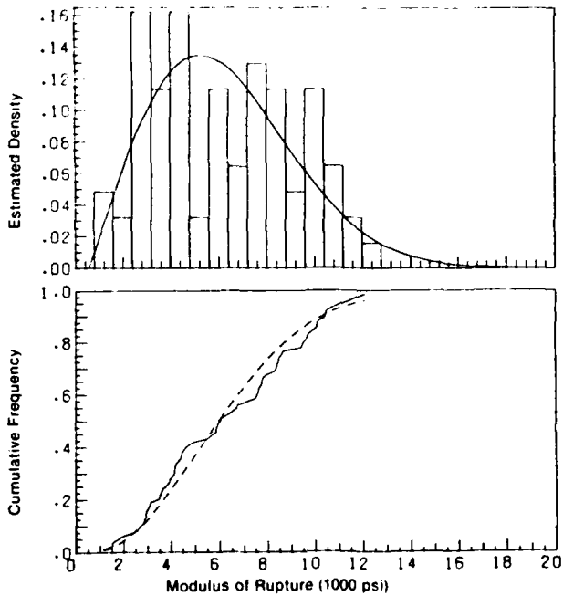
Figure A3.—Fit of three-parameter Weibull distribution to bimodal data (2 by 8, No. 3, 15 pct moisture content). (ML84 5324)
