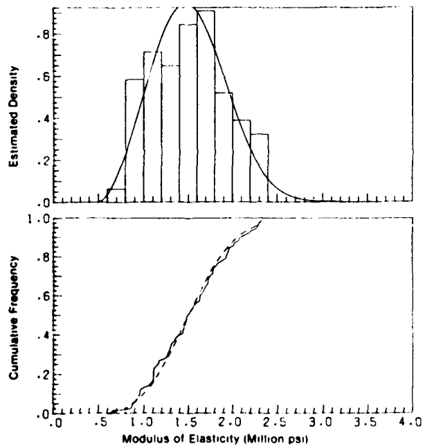
Figure A2.—Typical fit of three-parameter Weibull distribution to MOE data (2 by 8, No. 3, 15 pct moisture content). (ML84 5323)
