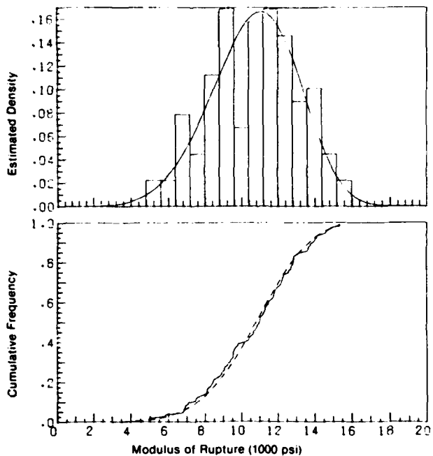
Figure A1.—Typical fit of three-parameter Weibull distribution to MOR data (2 by 4, Select Structural, 15 pct moisture content). (ML84 5322)
