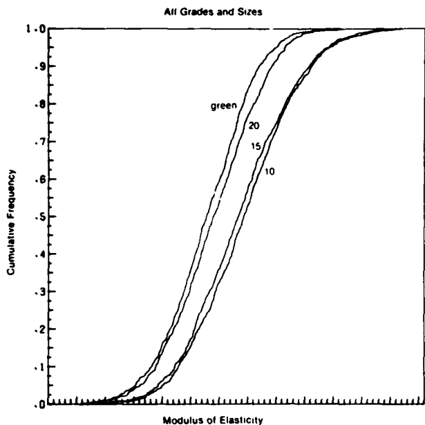
Figure 6.—Form of the cumulative frequency distributions of MOE for target moisture contents of 10, 15, and 20 percent, all grades and sizes combined. (ML84 5321)
