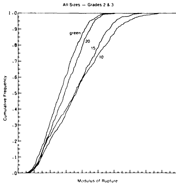
Figure 3.—Form of the cumulative frequency distributions of MOR for No. 2 and No. 3 grade lumber combined. (ML84 5319)
