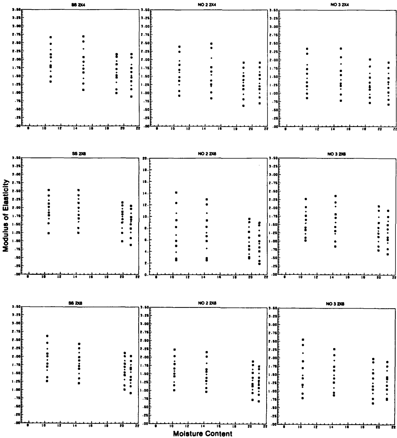
Figure B6.—Effect of moisture content on modulus of elasticity ( 10^4 psi) at various percentile levels (5, 10, 20...80, 90, 95). Percentiles plotted at average moisture content for the group (21 pct for green). (ML84 5264)
