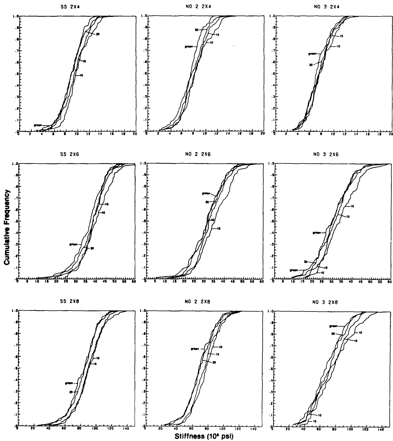
Figure B4.—Cumulative frequency distribution for EI at four moisture content levels. (ML84 5263)
