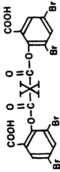
BIS-3,5-DIBROMOSALICYLIC ACID
