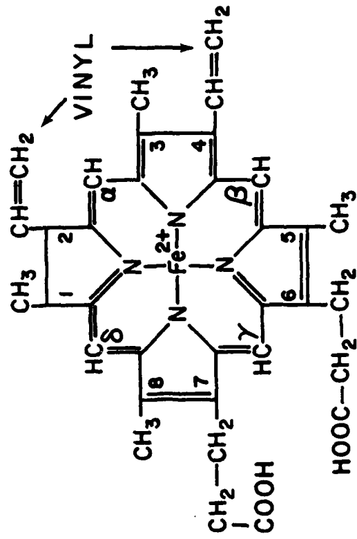
Ferroporphyrin-IX (heme)
