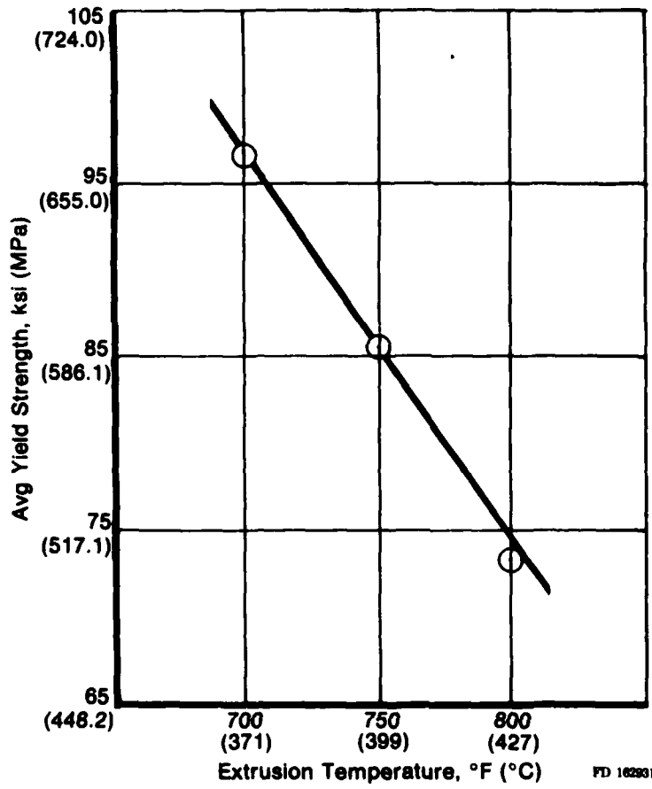
Figure 13. Effect of Extrusion Temperature on Yield Strength
