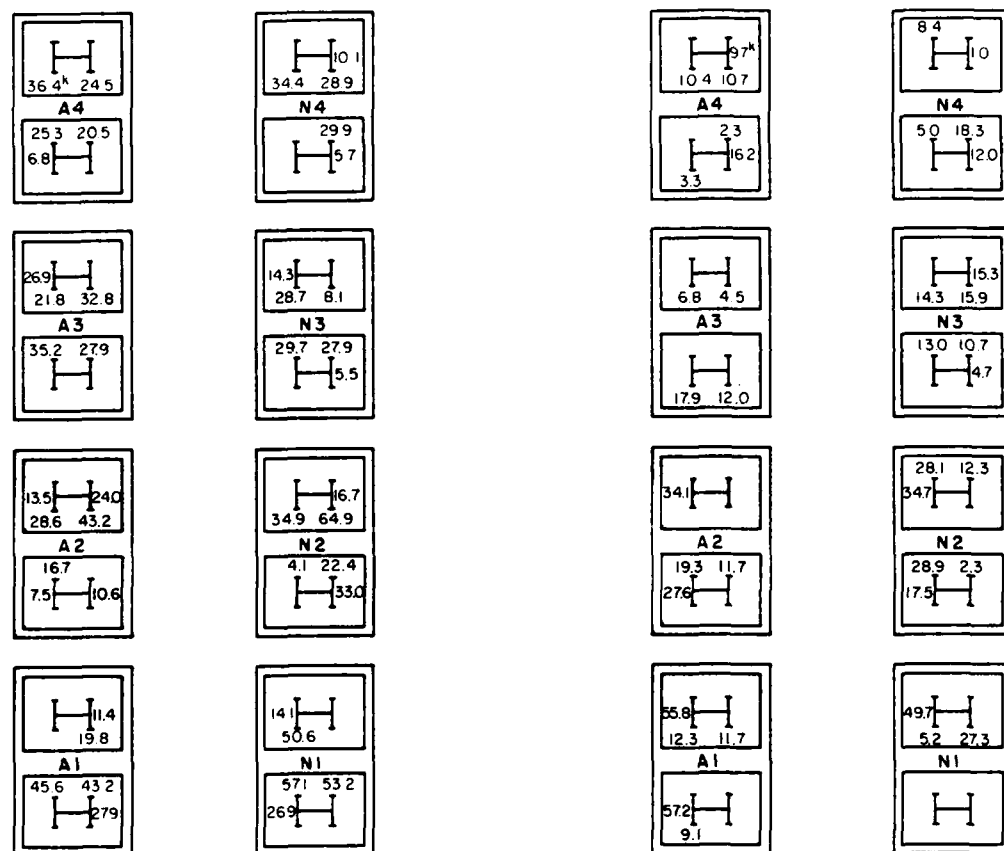
a. Building level. b. Level 1. Figure A2. Individual sway bolt load measurements (in kips [1000 lb]).
