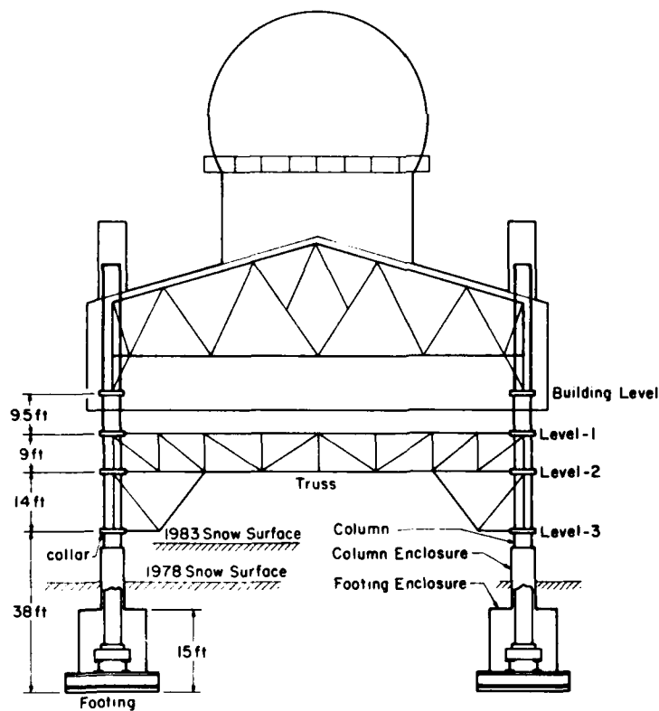
a. Elevation cross section.
