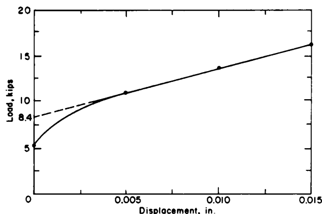
Figure 11. Typical load-displacement curve for a sway bolt that could not be backed off.
