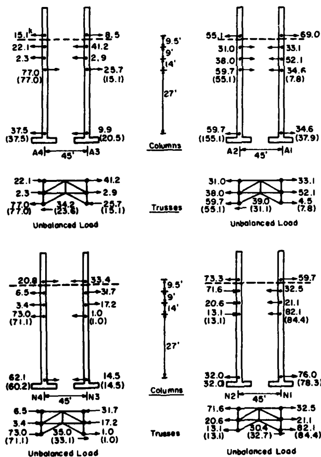
Figure B2 (cont'd). 1981 (values in parentheses were measured without friction-reducing devices).
