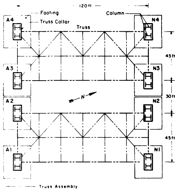
Figure 3 (cont'd). DYE-3 structural system.
