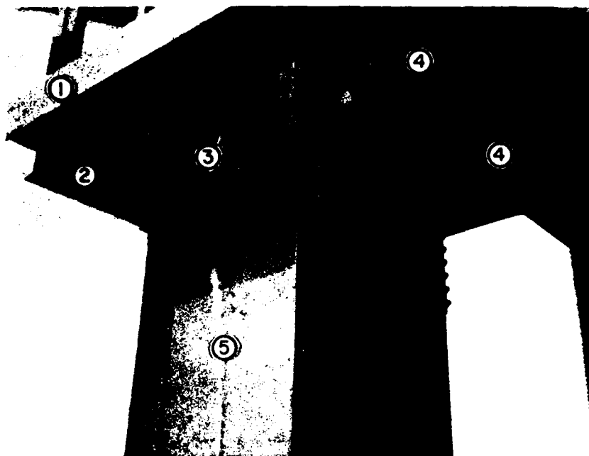
Figure 5. Truss support points and collar assembly (1 - collar, 2 - channel that supports truss, 3 - sway bolt [1 of 12 at each collar], 4 - beams that support truss, 5 - column half).
