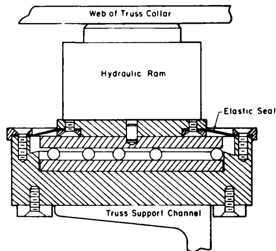
Figure 12. Cross section of friction-reducing roller devices.
