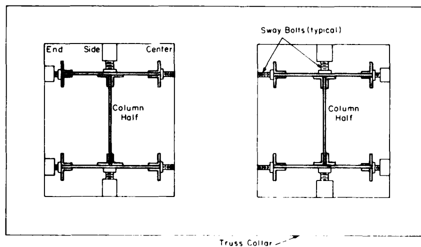
Figure 6. Plan view of typical truss collar and column showing the 12 sway bolts.
