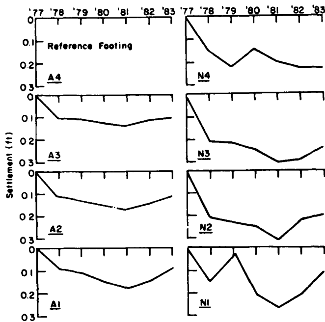
Figure 14. Footing settlements relative to footing A4, 1977-83.
