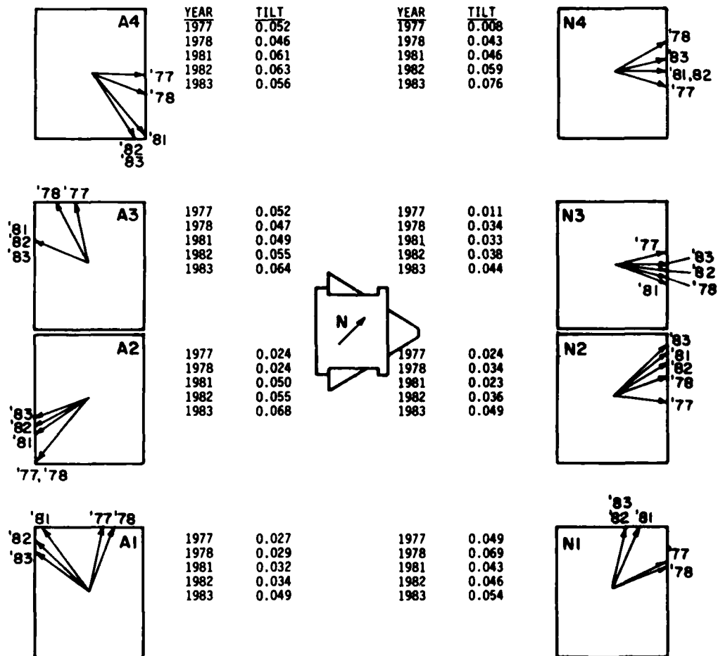
Figure 15. Footing tilts, 1978-83 (in./ft). Arrows indicate downward tilt directions.
