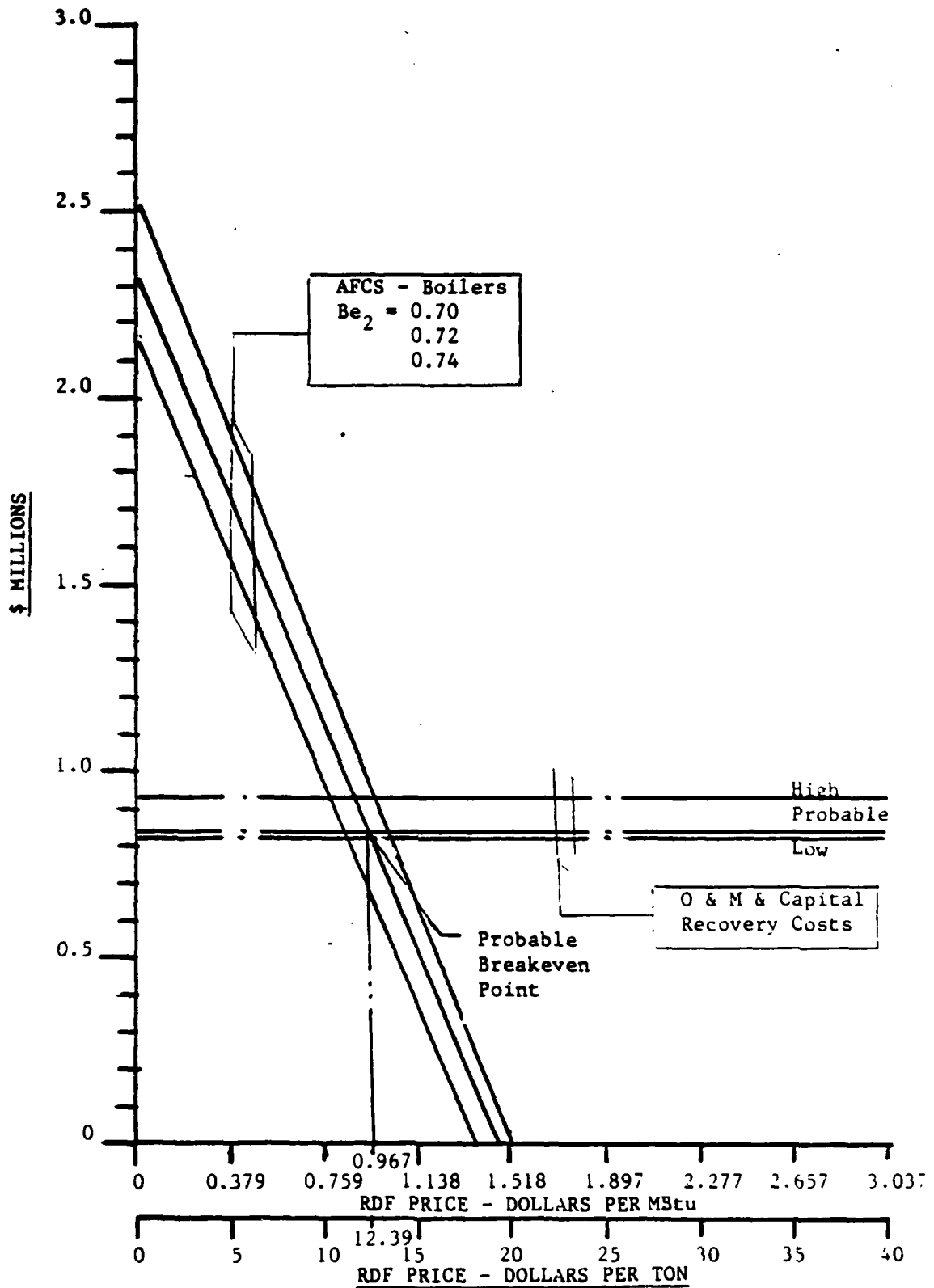
Figure C-4. Comparison of Annual Fuel Cost Savings to O&M, RDF, and Capital Recovery Cost for a Boilers Capacity of 300 MBtu/hr (2-150 MBtu/hr Boilers).
