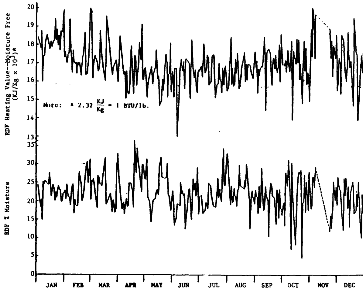
Figure 4-2. Daily RDF Moisture and Heating Values at Ames Municipal Power Plan - 1976 4 .
