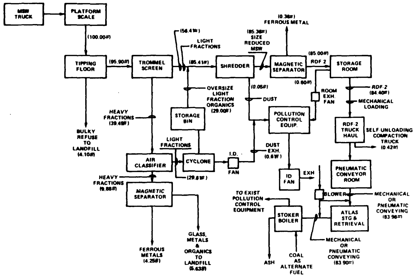
Figure 4-4 Flow Diagram of an MSQ Processing Plant to Produce RDF-2 Fuel.
