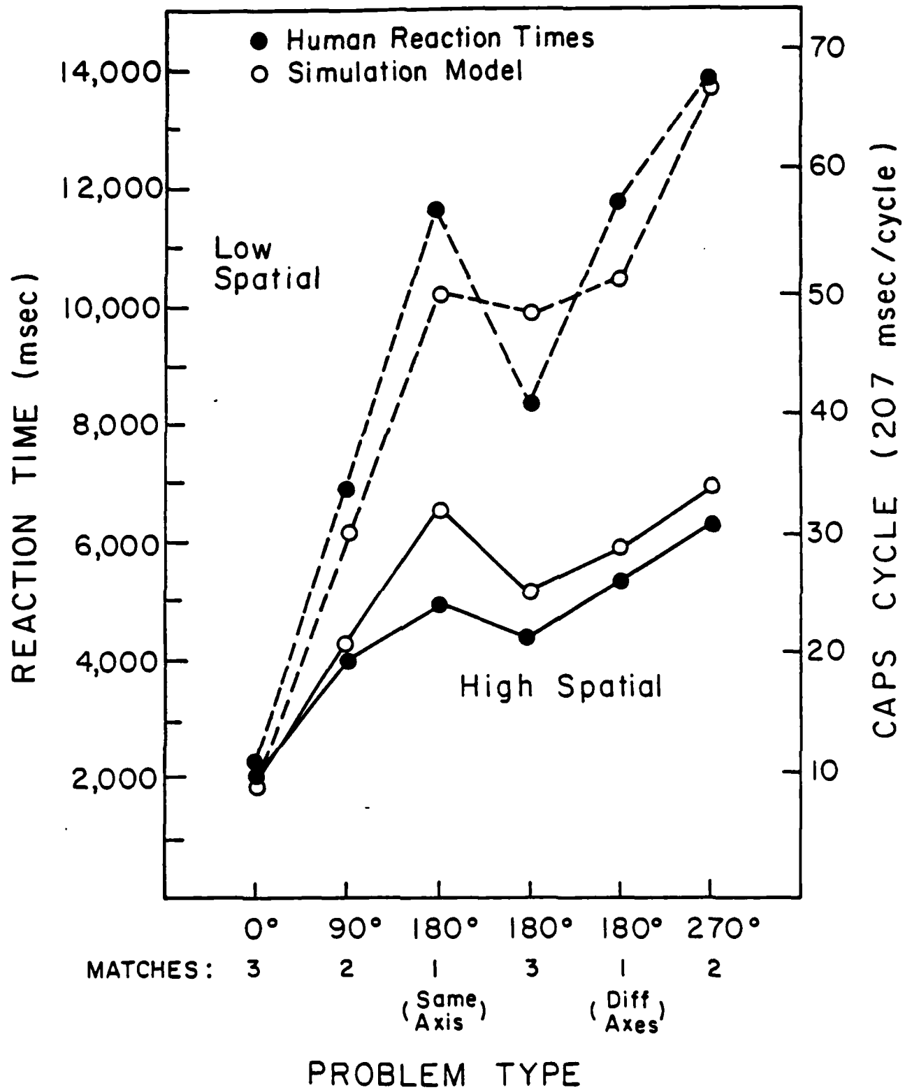
Figure 6. Human reaction times (left axis) and simulation model cycles (right axis) in the Cube Comparisons task.
