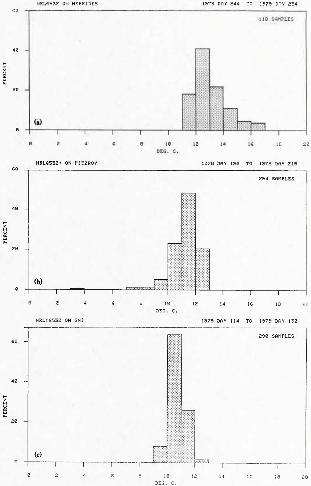
Fig. 7 — Temperature frequency-of-occurrence. (a) South Uist, (b) Open sea (57°N 20°W), and (c) San Nicolas Island.
