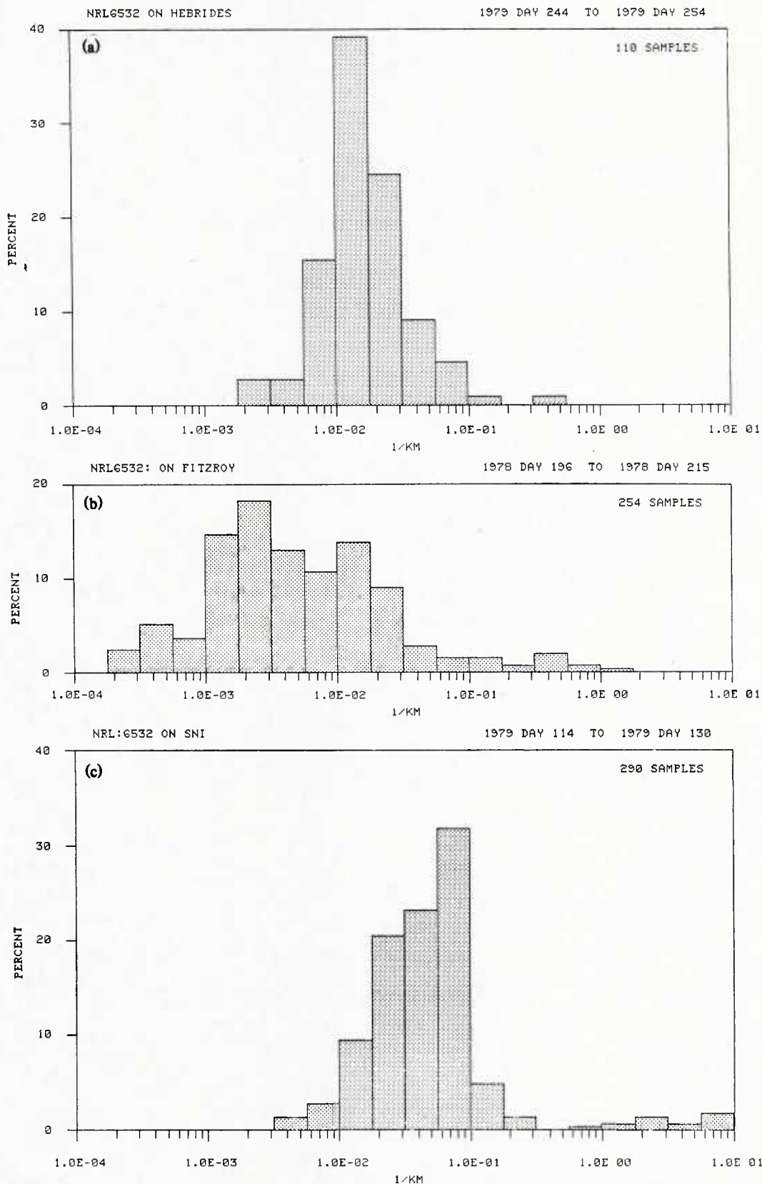
Fig. 12 — Calculated aerosol extinction at 10.6 μm frequency-of-occurrence. (a) South Uist, (b) open sea (57°N 20°W), and (c) San Nicolas Island.
