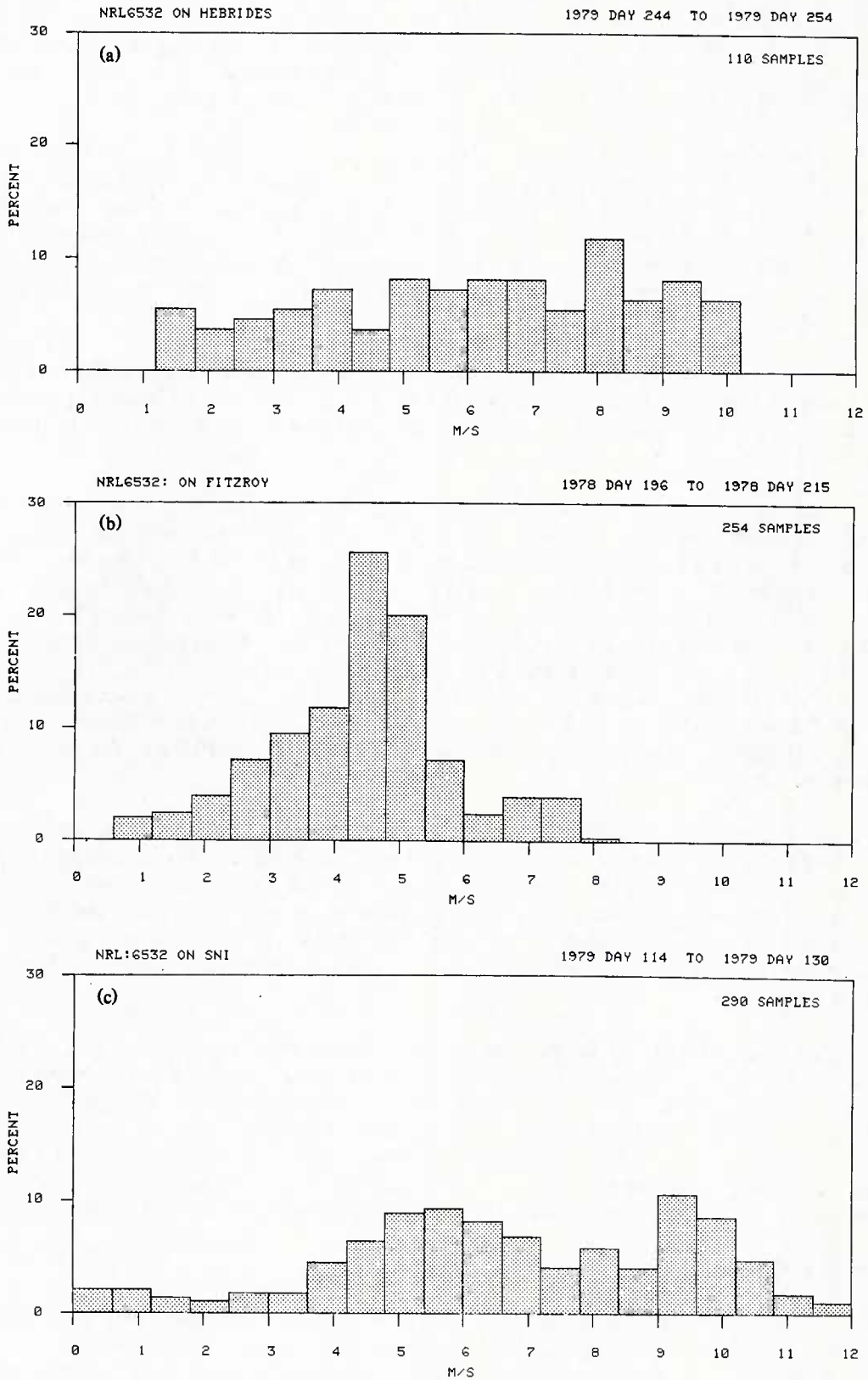
Fig. 9 -- Wind speed frequency-of-occurrence. (a) South Uist, (b) Open sea (57°N 20°W), and (c) San Nicolas Island.
