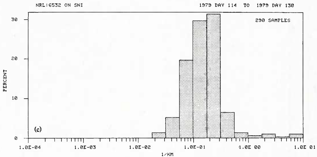
Fig. 11 — Calculated aerosol extinction at 3.8 \mu m frequency-of-occurrence. (a) South Uist, (b) open sea (57°N 20°W), and (c) San Nicolas Island.
