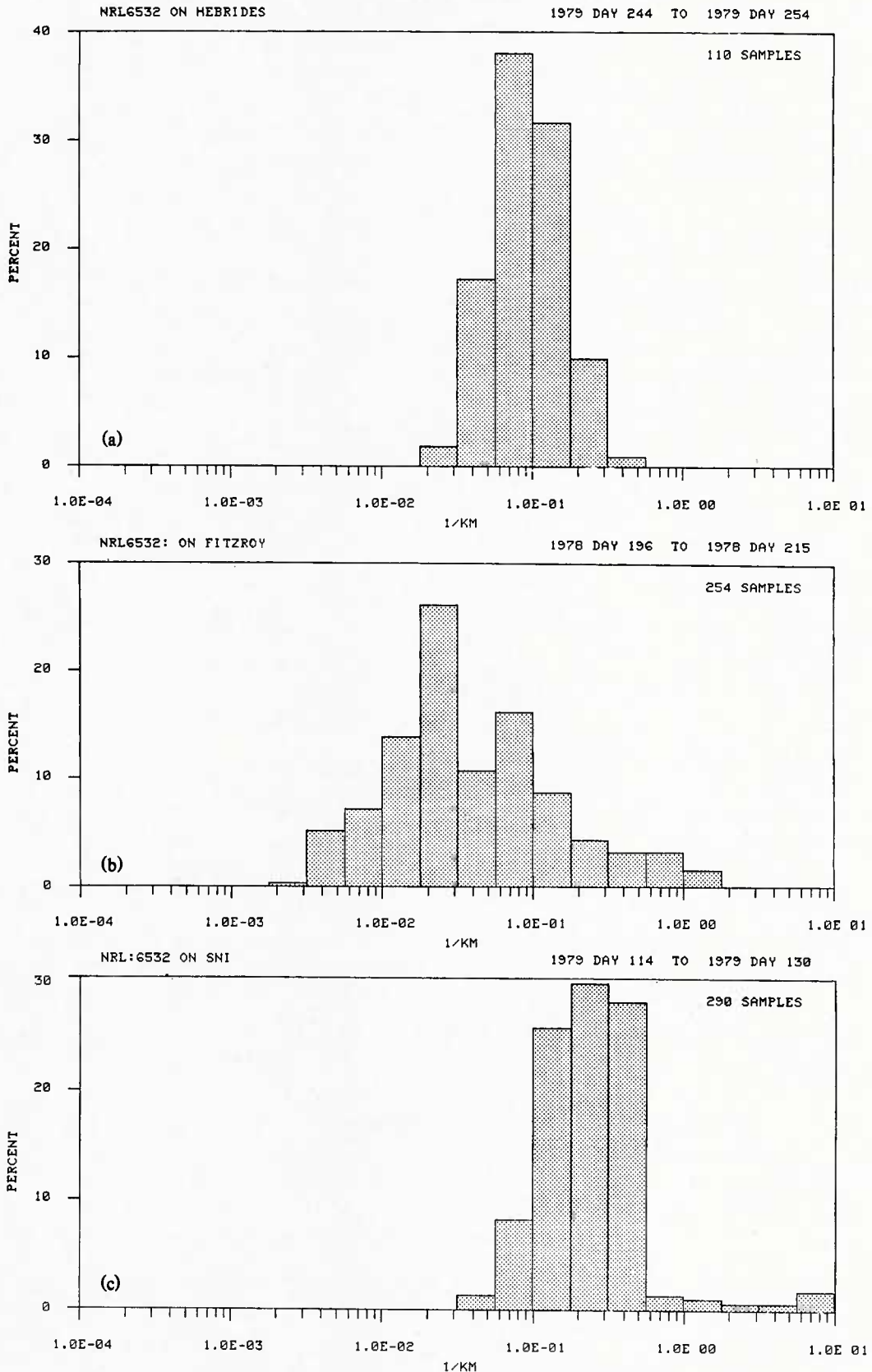
Fig. 10 - Calculated aerosol extinction at 0.55 \mu\text{m} frequency-of-occurrence. (a) South Uist, (b) open sea (57°N 20°W), and (c) San Nicolas Island.
