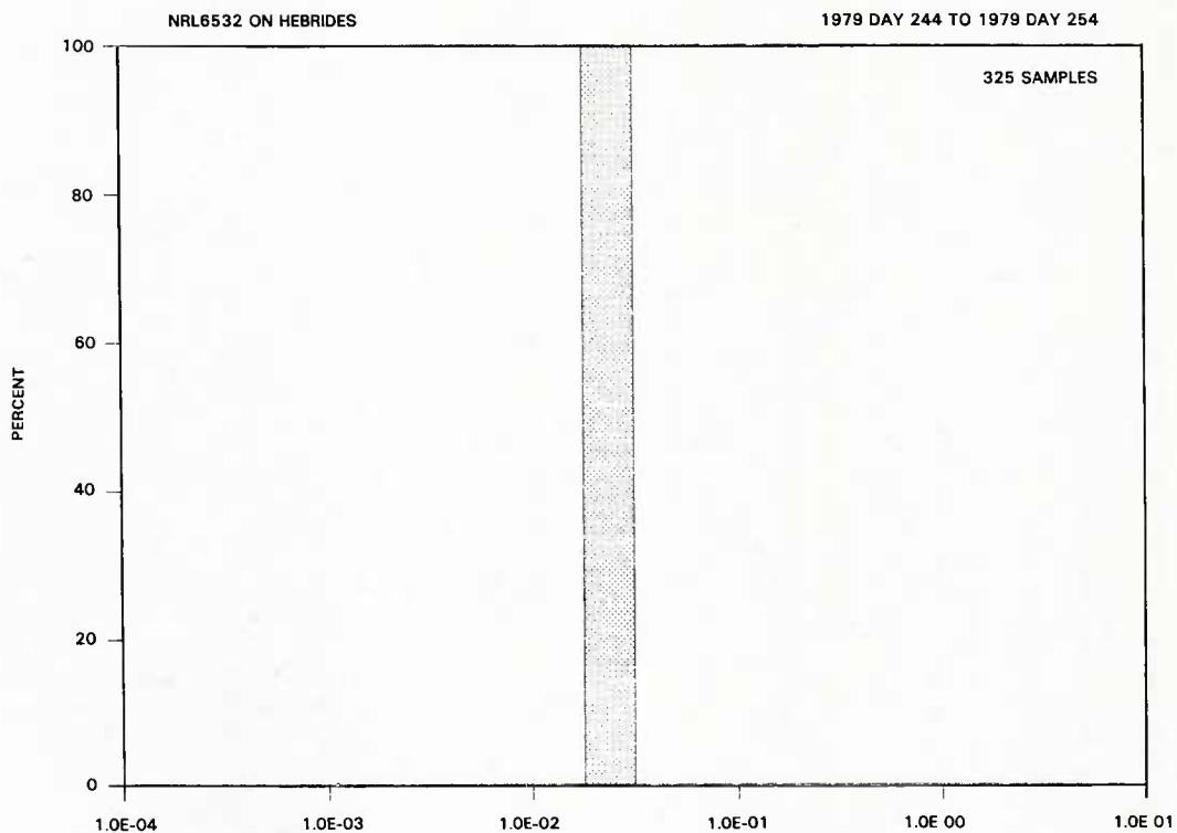
Fig. 13 — Calculated molecular absorption at the P_2(8) DF Laser frequency, frequency-of-occurrence
