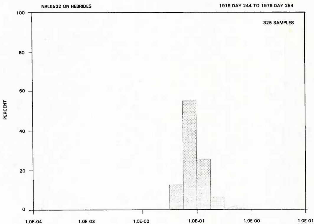
Fig. 14 — Calculated total extinction at the P_2(8) DF Laser frequency, frequency-of-occurrence
