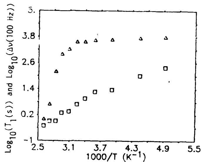
Fig. 2. Temperature dependences of 7 Li FWHM linewidth (Δ) and effective T 1 (□).
