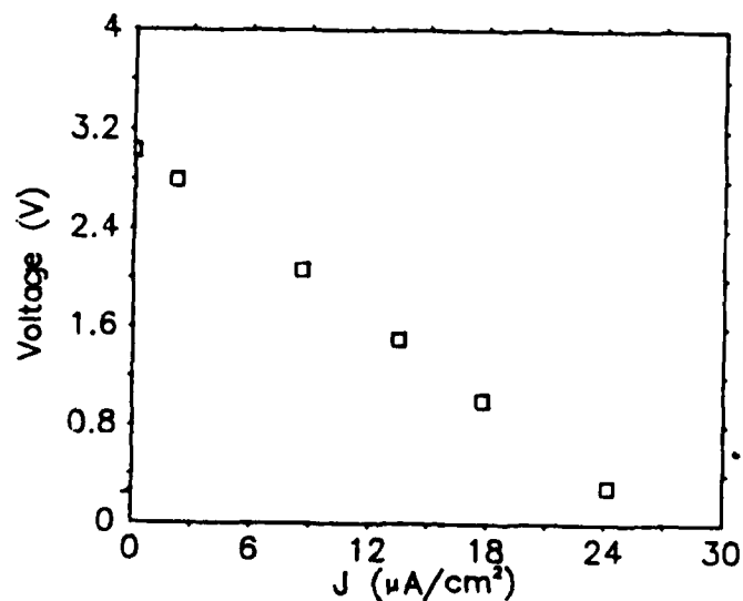
Fig. 3. Voltage (V) vs. J(μA/cm 2 ) for the cell: Li/PVAcg-LiClO 4 /MnO 2 -C-PVF 2 at 125°C.
