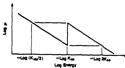
FIG. 7 - Variation of the linear attenuation coefficient \mu at the K_{\alpha b} photoelectric absorption edge.
