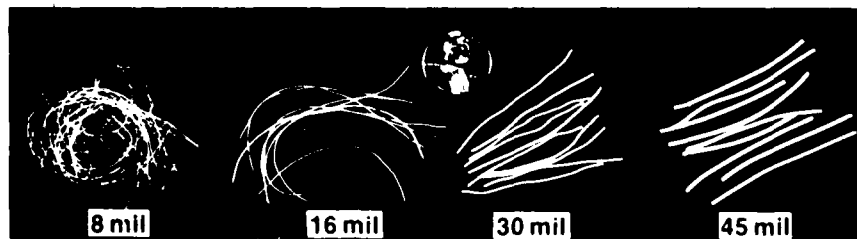
Figure 1. Controlled-release PCL fibers containing fluridone (26 percent a.i. by weight). NOTE: Smaller diameter fibers curl more than larger diameter fibers
