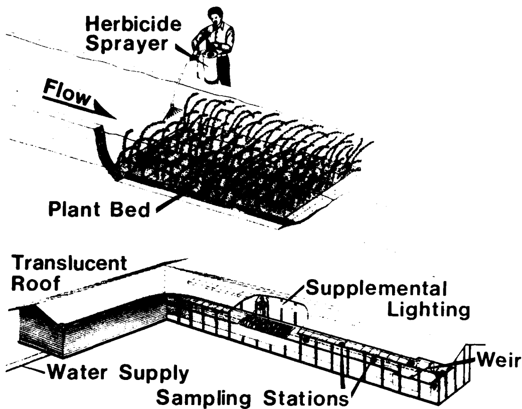
Figure 1. Flume system set up to evaluate the effectiveness of herbicide/adjutant mixtures in controlling aquatic plants growing in flowing water
