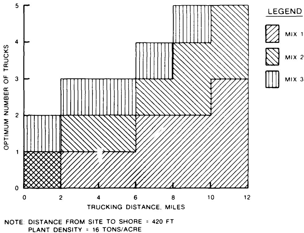
Figure 6. Optimum number of trucks by mix for variable trucking distances
