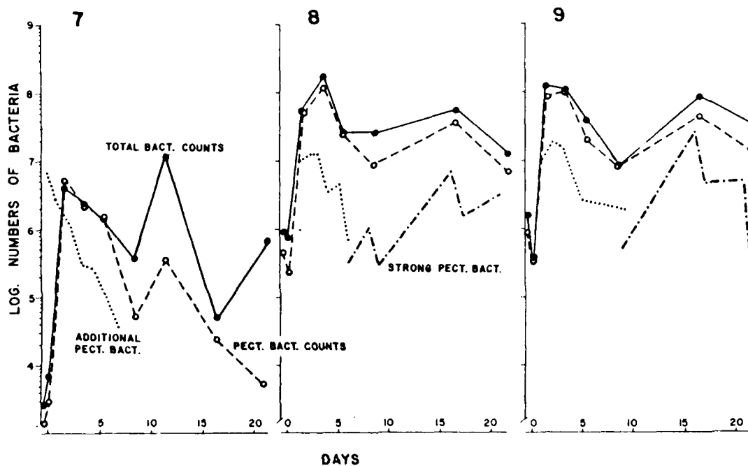
Figure 7. Effect of the addition of a selected pectinolytic bacterium YP-4 on bacterial populations recovered per millilitre of angiosperm medium supporting M. heterophyllum to which \alpha - naphthaleneacetic acid has been added
