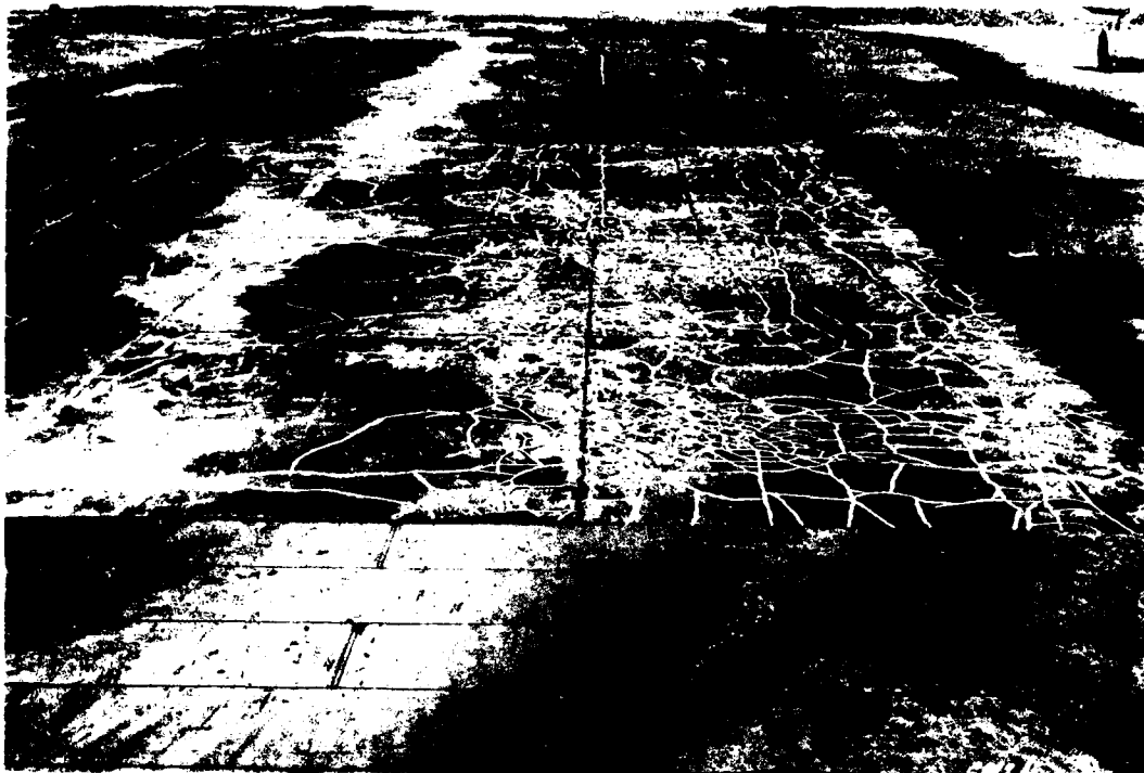
Photo 29. Item 6 after 2500 passes and 500 turning movements
