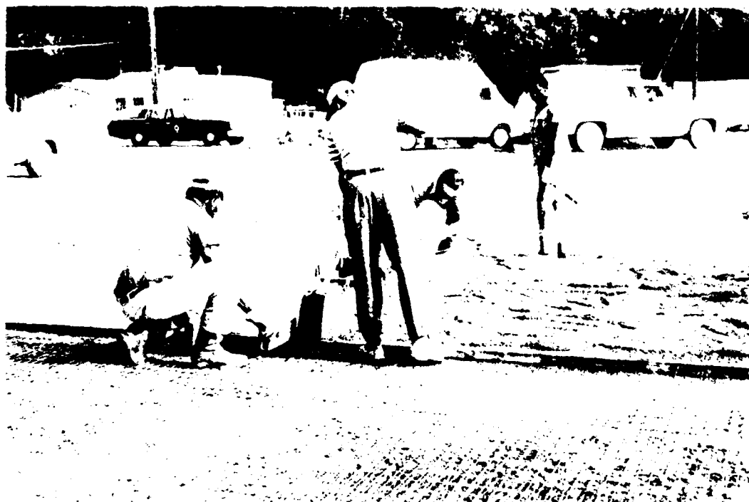
Photo 3. Placing concrete in item 1
