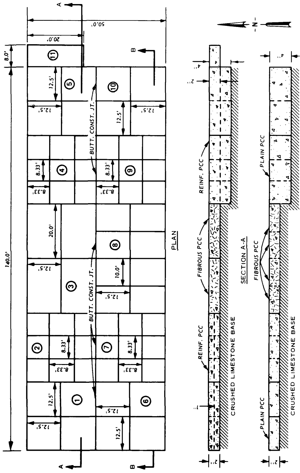
Figure 1. Plan and layout of test section
