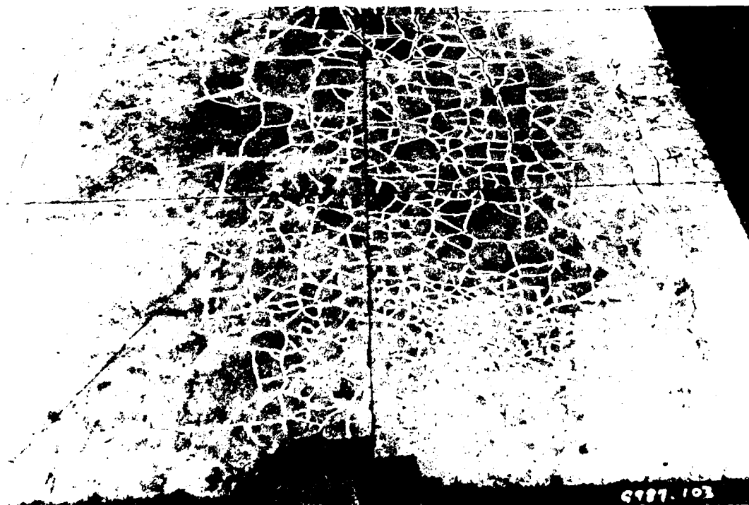
Photo 40. Item 6 after traffic tests were completed
