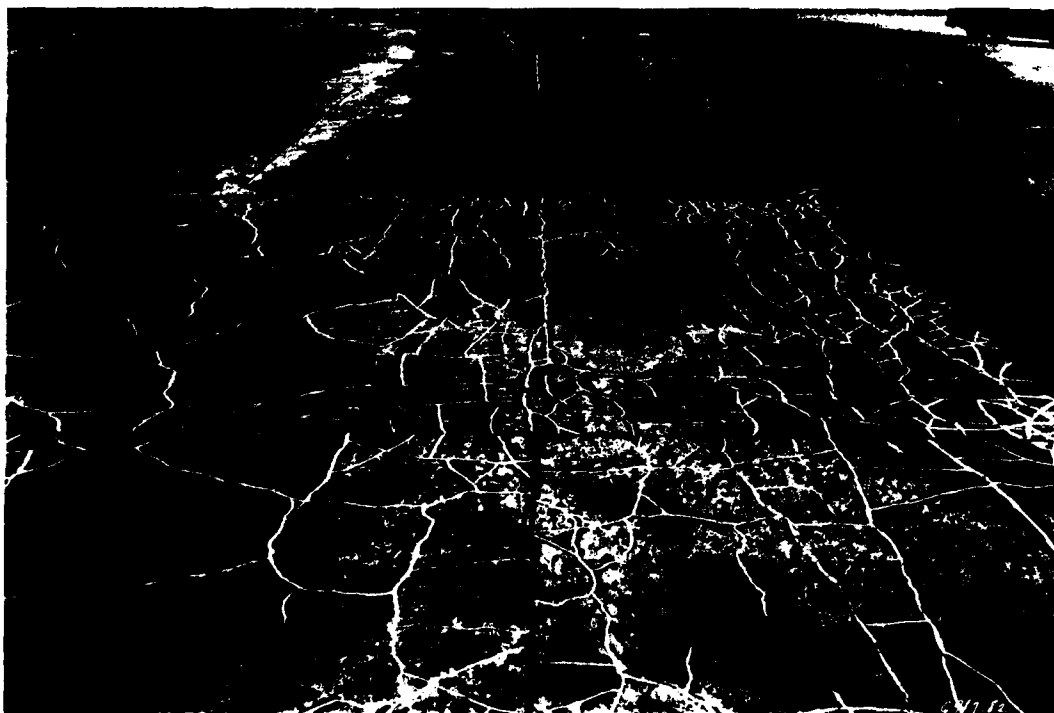
Photo 30. Item 7 after 2500 passes and 500 turning movements
