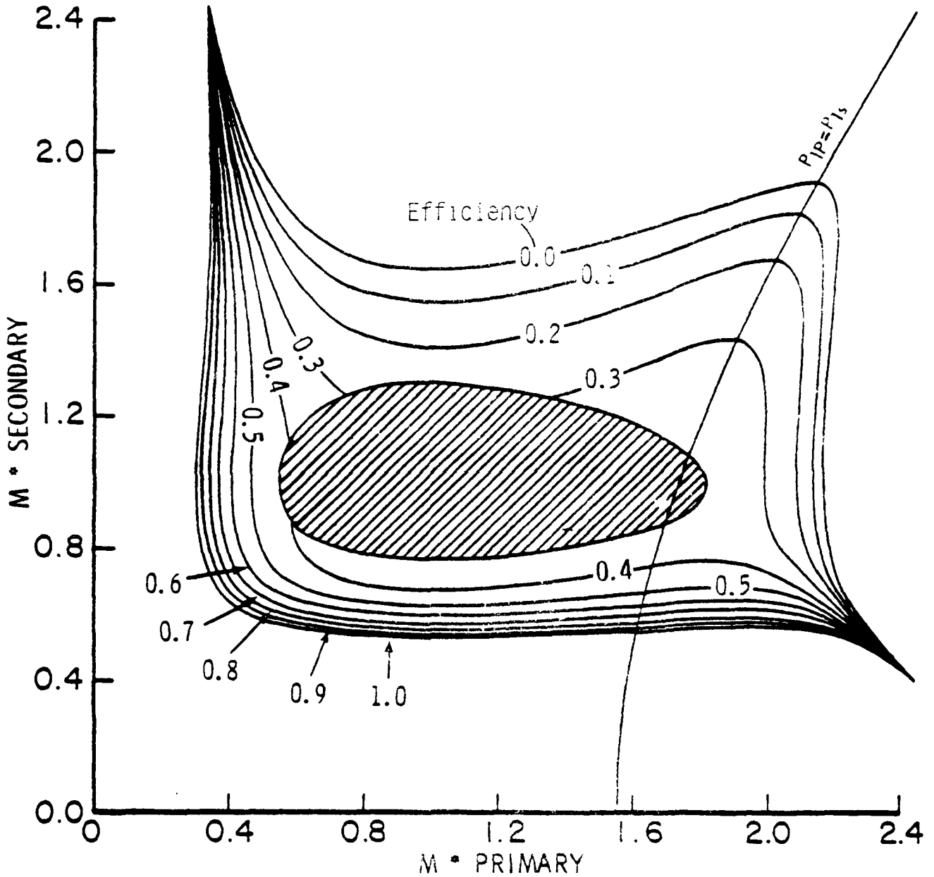
Figure 3. Supersonic Branch Efficiency Map. Also Shown is the Curve for which P_{1p} = P_{1s} . The Curve is a Design Curve Because the Physical Size of the Ejector Has to Change as One Moves Along the Curve.
