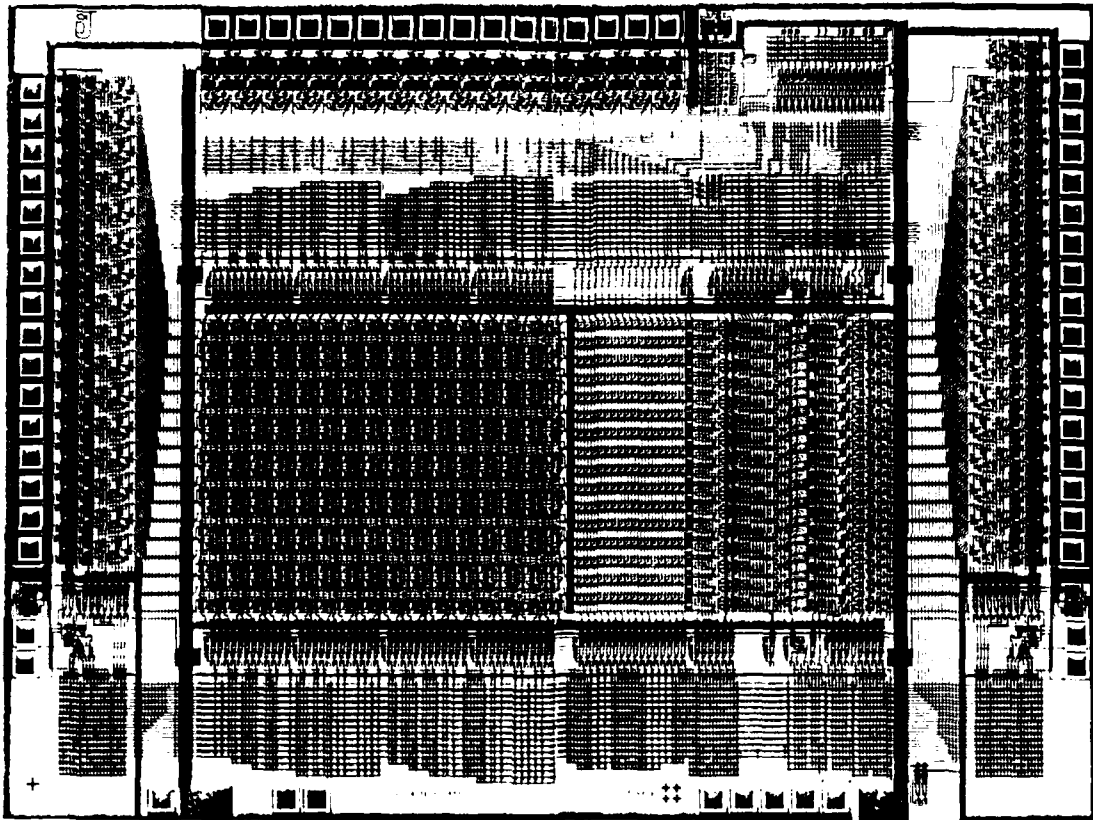
UNCLASSIFIED Figure 8 CALTECH'S data path chip
