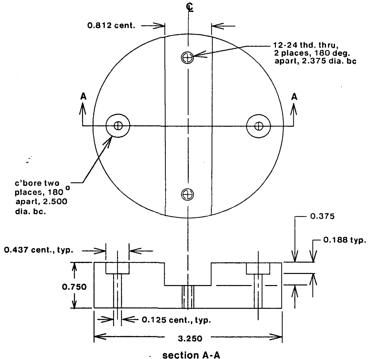
Figure 3-1: Typical Finished Part Made From Bar-Stock
