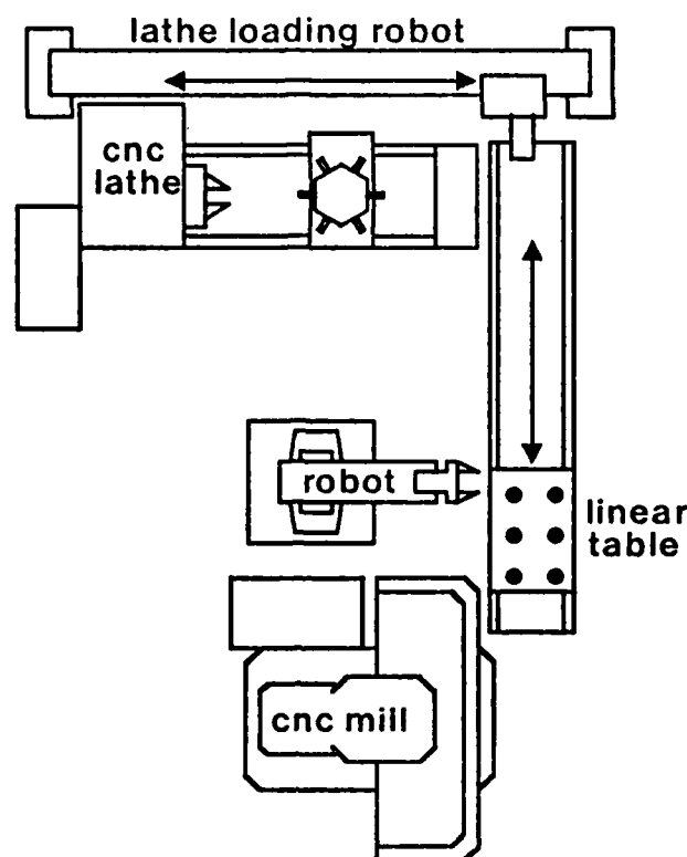
Figure 3-2: Machining Cell Layout -- First Arrangement
