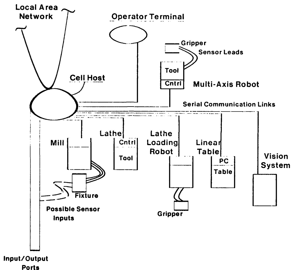
Figure 3-5: Cell Host-Controller Communication Scheme
