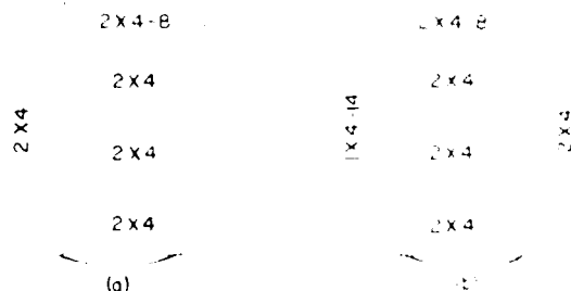
Figure 7.—Smaller dimension product allows increase in lumber recovery on a 7.1-inch-diameter 16-foot-long log (Pieces cut to less than full log length have their length indicated, those of full length show no length.) a) Standard dimension lumber—48 board foot yield b) Standard dimension lumber and 1 by 4's—52-2/3 board foot yield (M152037)
