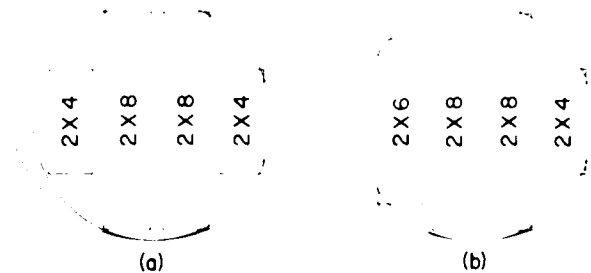
Figure 4.—Shift in pattern due to reduced kerf allows wider lumber to be cut from 8.3-inch-diameter 16-foot-long log. a) 0.240-inch kerf—64 board foot yield. b) 0.180-inch kerf—69-1/3 board foot yield. (M152041)
