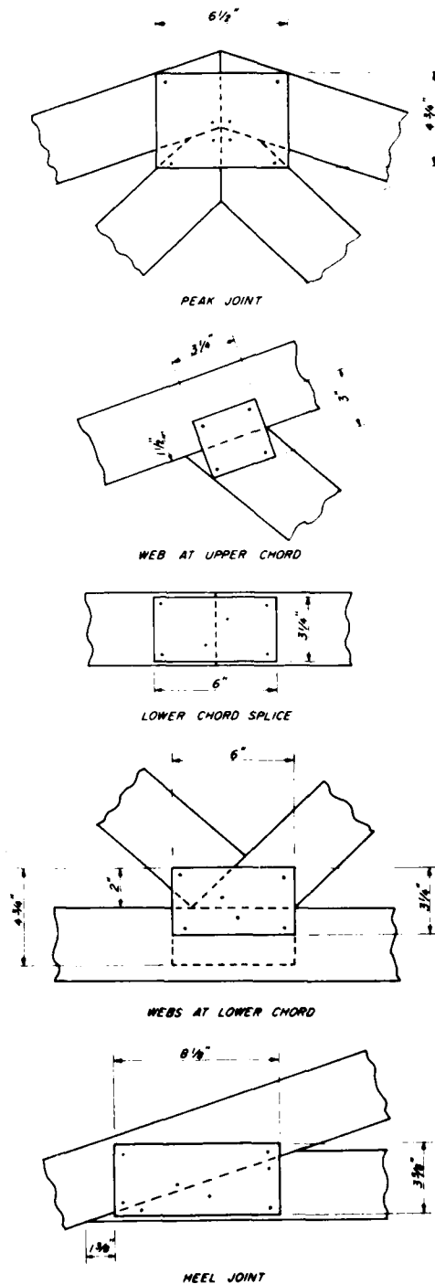
Figure 6.—Joint details for barbed metal plate trussed rafters. Plates were 20-gage galvanized sheet metal. Positioning nails were 1-1/2-inch-long annular-grooved nails. (M134832)
