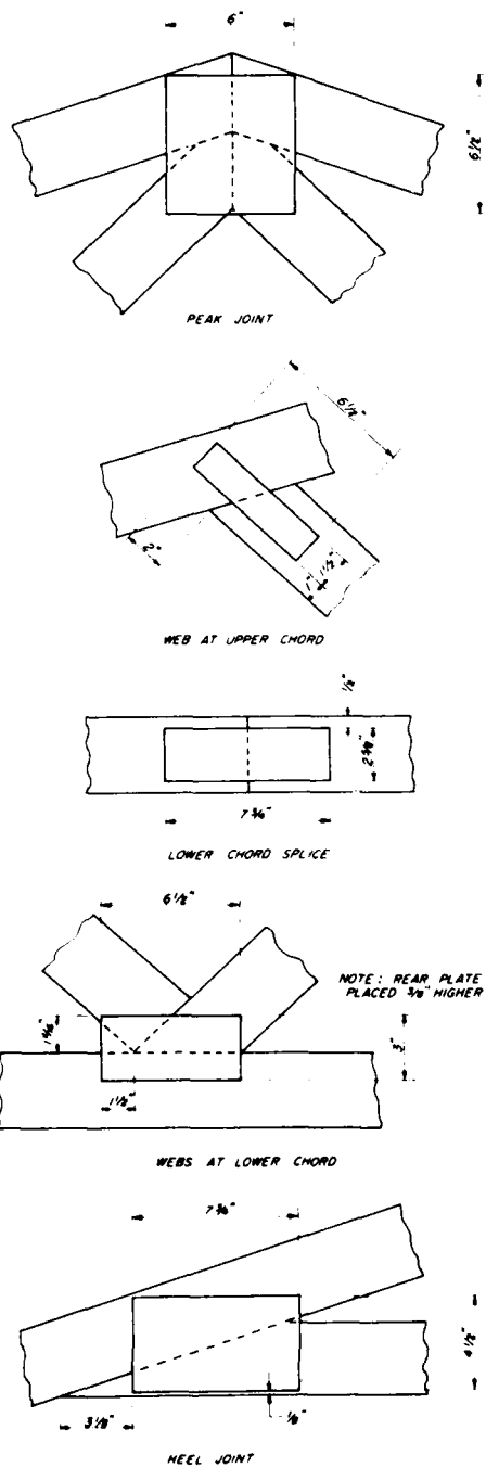
Figure 5.—Joint details for toothed metal plate trussed rafters. Plates were 18-gage galvanized sheet metal with 3/4-inch-long teeth. (M134835)
