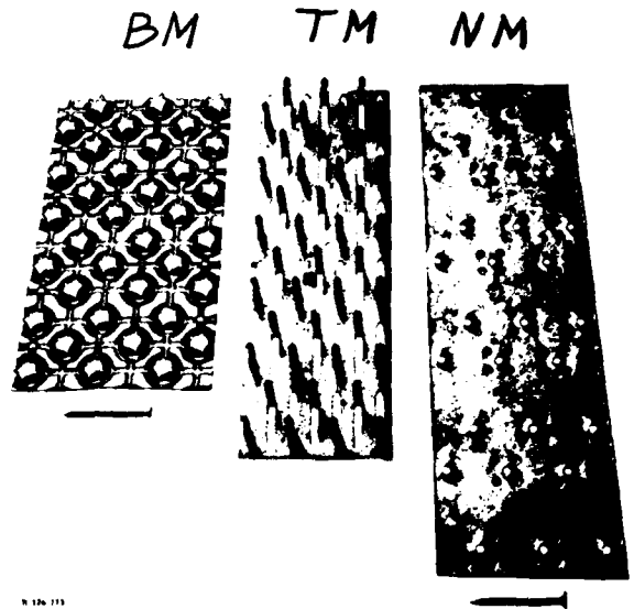
Figure 2.—Three types of metal plates selected for the longtime performance study. Left, barbed metal plate (20-gage); center, toothed plate (18-gage); and right, nailed metal plate (20-gage). (M124773)
