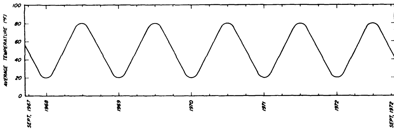
Figure 20.—Average temperatures inside the pole building during the first 5 years of trussed rafter loading. (ML835520)
