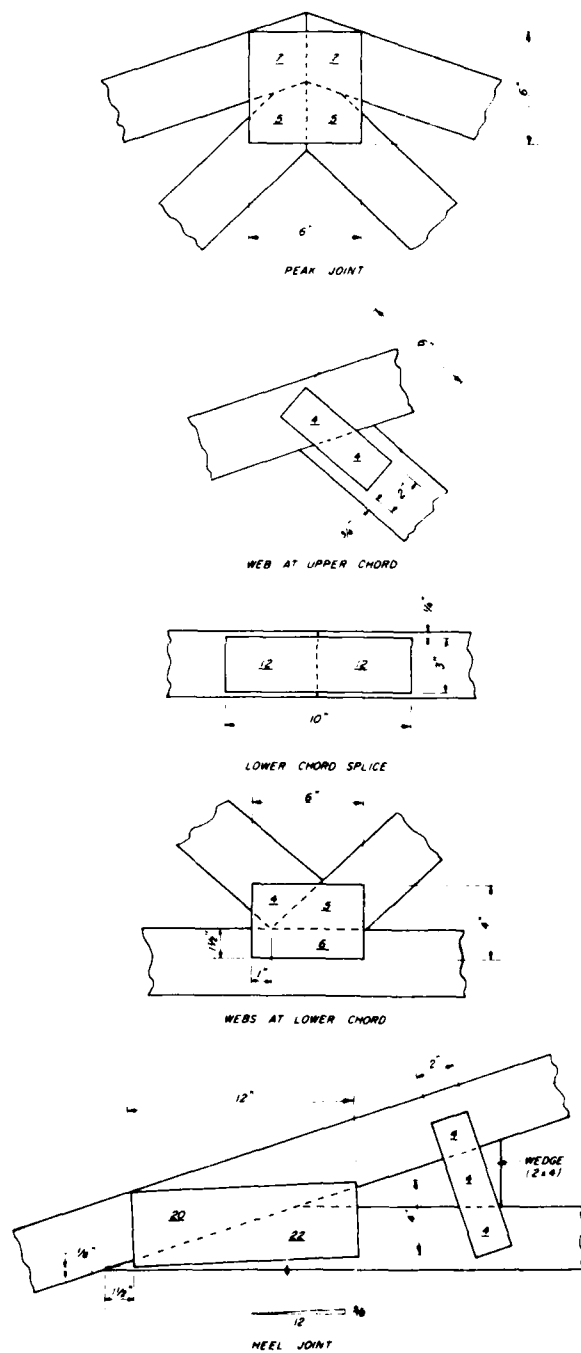
Figure 4.—Joint details for nailed metal plate trussed rafters. Numbers on gussets refer to the number of nails used. Nails were 1-1/2-inch-long annular grooved. Gussets were 20-gage galvanized sheet metal with punched holes. (M134836)
