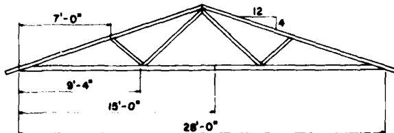
Figure 1.—Details of truss member location. All members are nominal 2 by 4's. (M140987)
