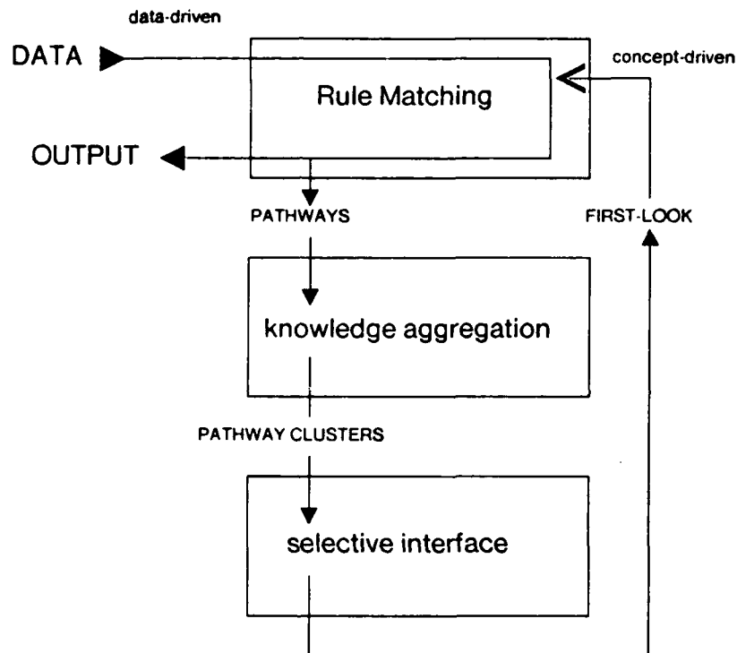
Figure 2-1: Modules and flow of information
