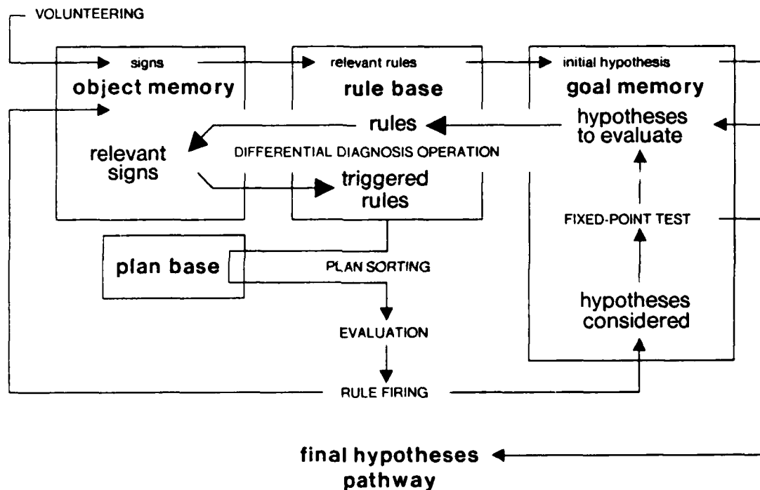
Figure 4-1: General mechanism of the NCLOSE algorithm
