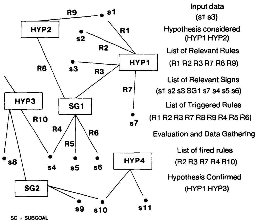
Figure 4-2: Simple model of propagation and control
