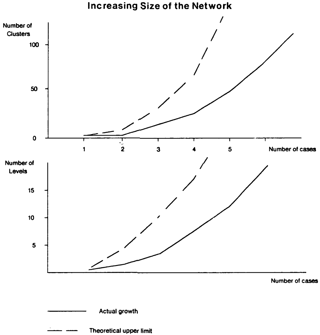
Figure 5-1: Actual vs Polynomial growth of network size
