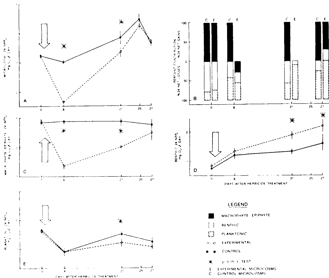
Figure 15. Changes in mean 24-hr net primary productivity (24 NPP): total microcosm 24-hr NPP (A), percent productivity contribution by each component (B), macrophyte-epiphyte 24-hr NPP (C), benthic 24-hr NPP (D), and planktonic 24-hr NPP (E). Bars represent standard errors and asterisks indicate significant differences ( p < 0.05 , t-test)
