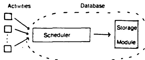
Figure 3-1: The scheduler model.
