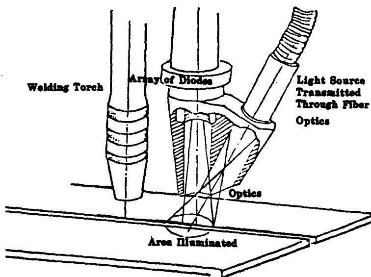
Fig. 2. Joint characterization by linear array of photodiodes.
