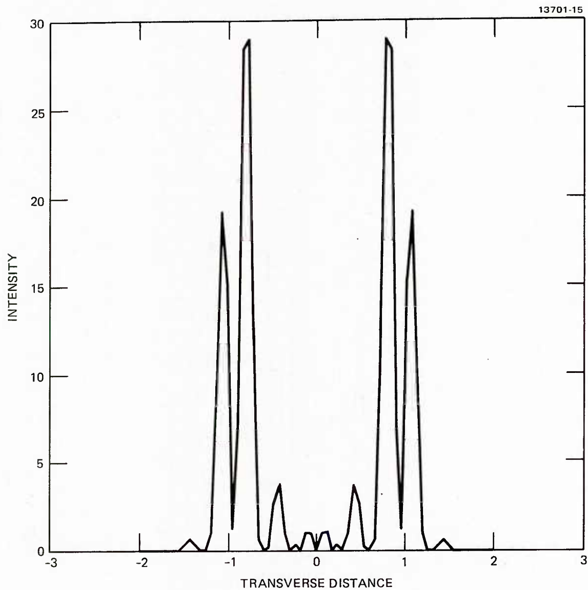
Figure 16. Intensity distribution for the case when the adjacent emitters are 180° out-of-phase and the separation between emitters is 10 μm. Transverse distance is measured in units of (\lambda f / 2\pi a_0) .
