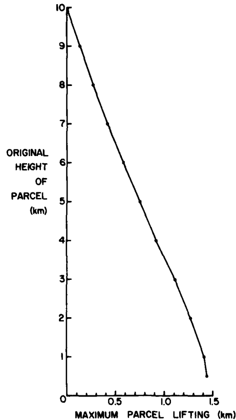
Figure 9. Lifting Experienced by Parcels During Gust Front Passage for Case QD5
