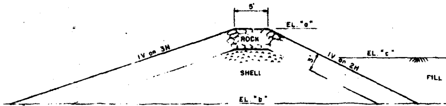
DIKE SECTION - REACHES W-III, E-I, E-II, E-III
