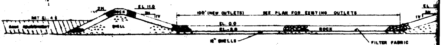
SECTION C-C
