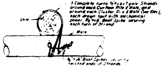
STRAND TIE SECURING PILE TO WALE
