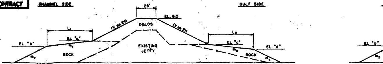
WEST JETTY SECTION
