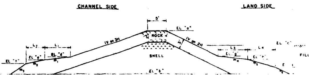
DIKE SECTION - REACHES W-X, E-II-A
