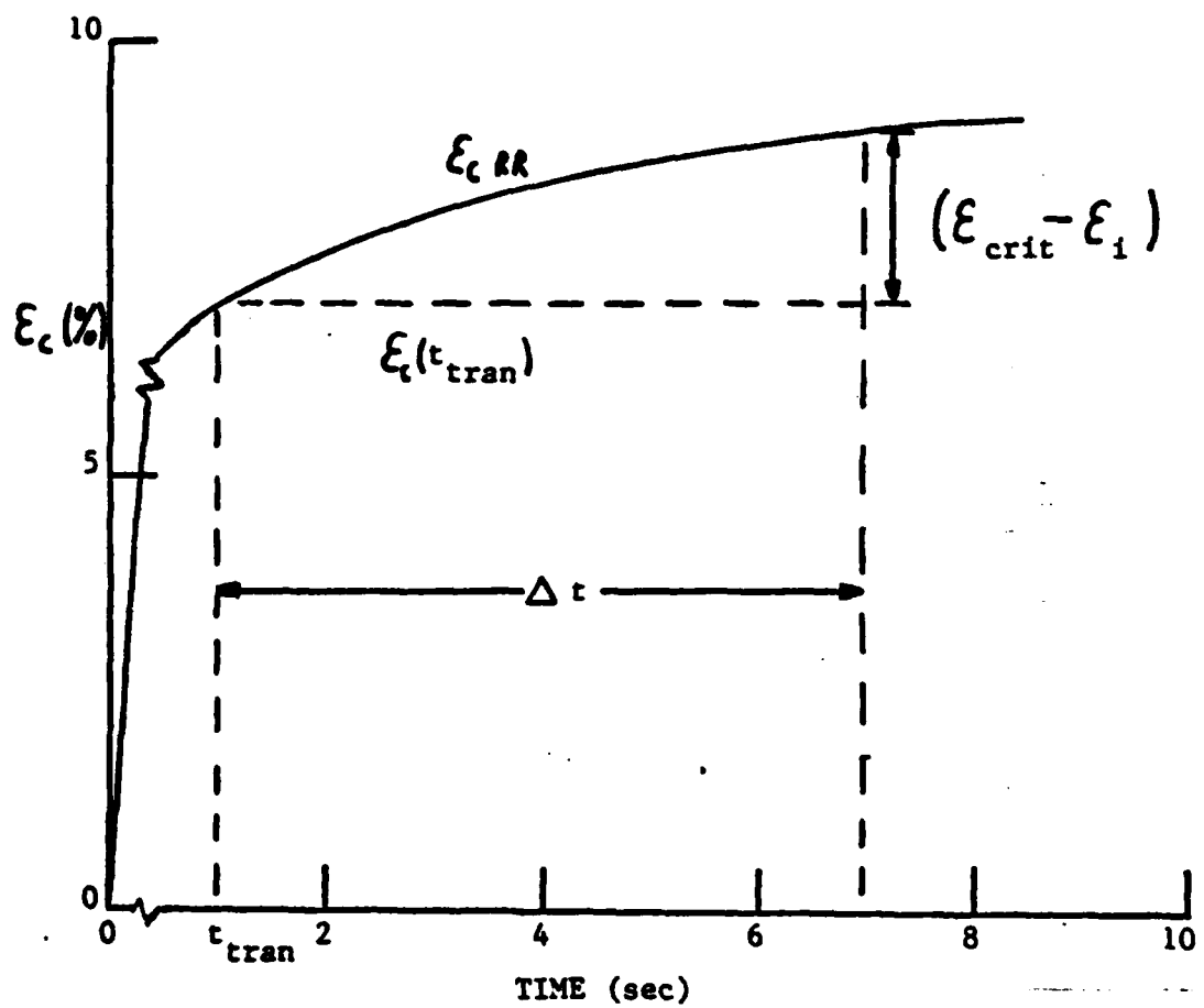
FIGURE (24) Schematic representation of the time for a crack advance in CCG, \Delta t .
