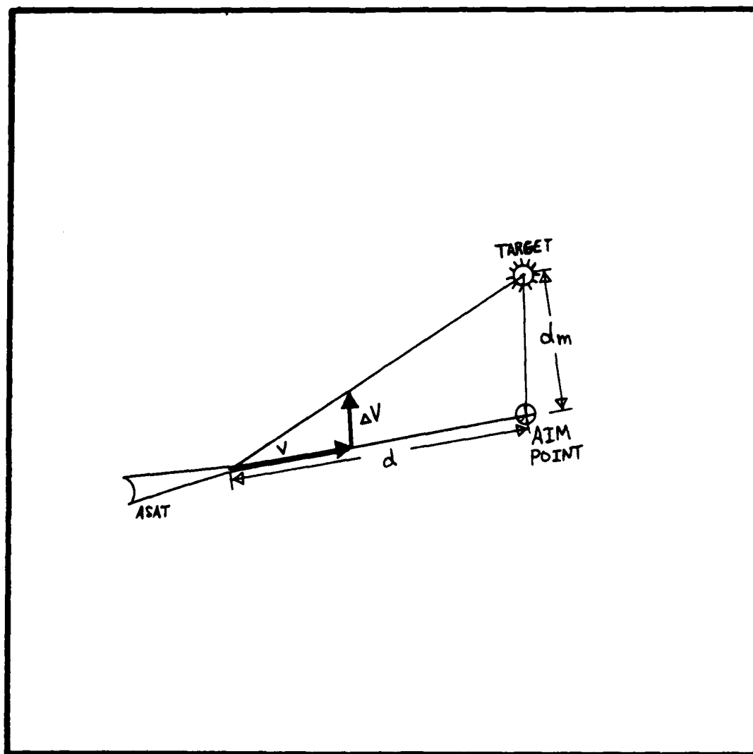
Figure 2-5. Similar Triangle Approximation for Delta V
