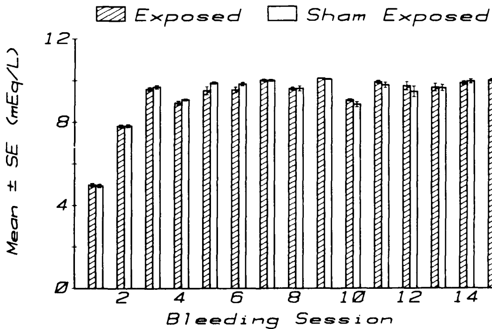
Fig. 20. Comparison of data on serum CHLORIDE for exposed and sham-exposed animals for 15 sampling sessions.
