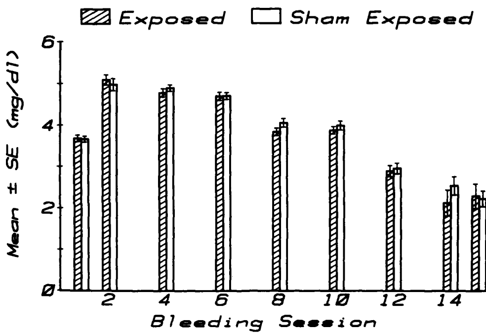
Fig. 39. Comparison of THYROXINE data for exposed and sham-exposed animals for sessions for which analysis was made.
