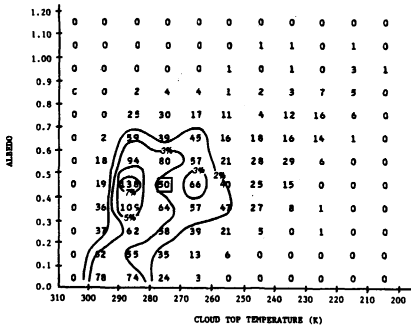
Figure 16. No-Precipitation Overcast Data for 8 x 8 Array Size (The mean, .411 and 272.5K, interval is boxed. The 2%, 3%, 5% and 7% frequencies are for 40, 59, 99, and 138 occurrences, respectively.)
