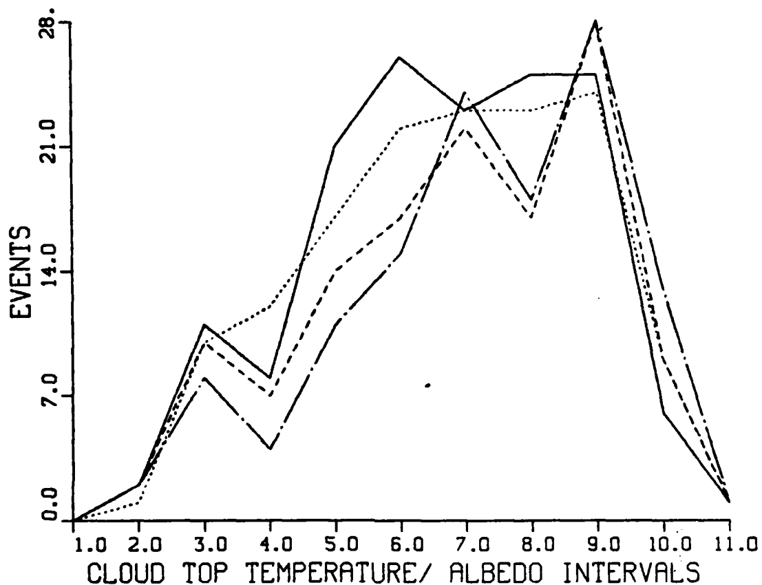
Figure 14. Precipitation Array Size Distributions Along Diagonal Line. (The line represents the 10 x 10, dotted line the 8 x 8, dashed line the 6 x 6, and dash dot line the 4 x 4 array size.)
