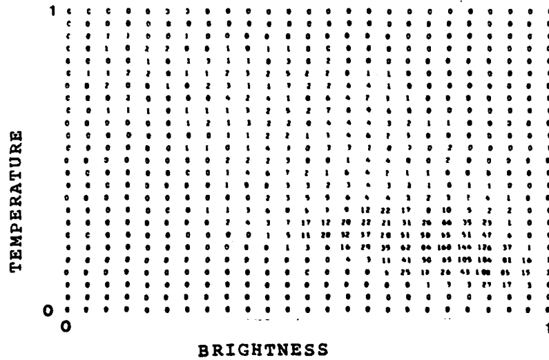
Figure 6. Frequency Plot of Rain Distribution for GATE day 248, 1300 GMT (from Lovejoy and Austin, 1979)
