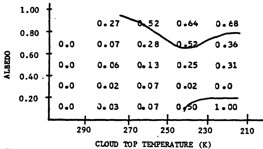
Figure 22. Precipitation Overcast Data Probability 4 x 4 Array Size
