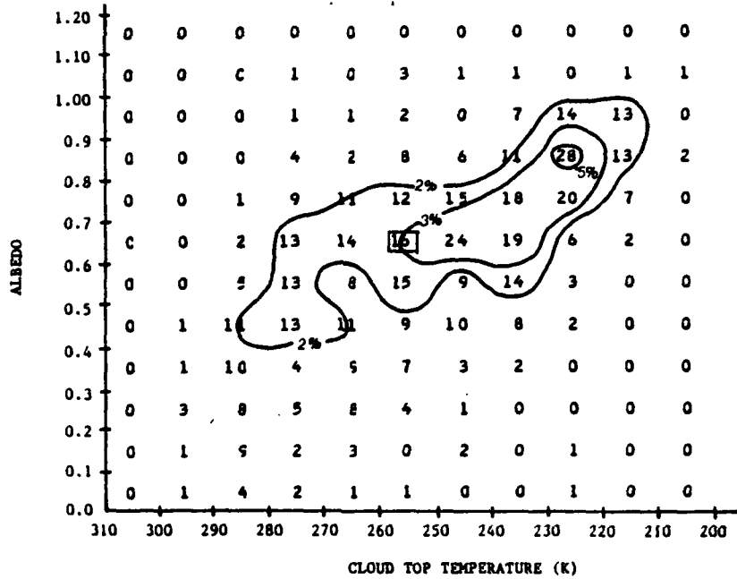
Figure 25. Precipitation Overcast and Broken Data for 4 x 4 Array (The mean, .616 and 250.6K, interval is boxed. The 2%, 3%, and 5% frequencies are for 11, 16, and 27 occurrences, respectively.)
