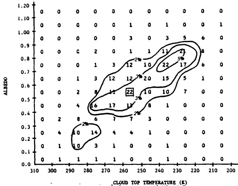
Figure 29. Convective Precipitation Data for 10 x 10 Array Size (The mean, .576 and 251.8K, interval is boxed. The 2%, 3%, and 5% frequencies are for 9, 13, and 21 occurrences, respectively.)
