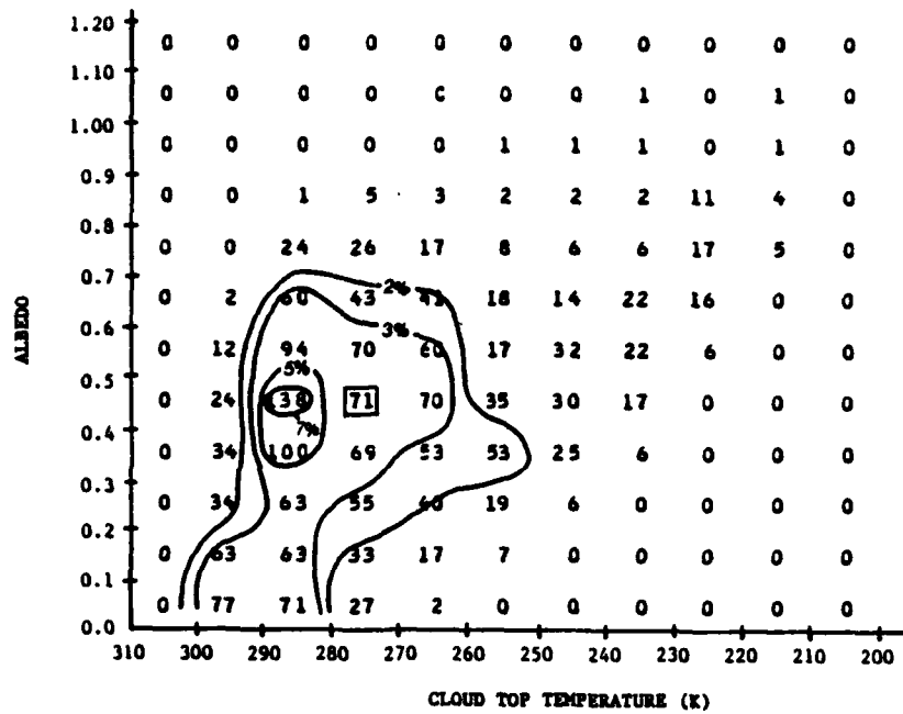
Figure 15. No-Precipitation Overcast Data for 10 x 10 Array Size (The mean, .407 and 272.6K, interval is boxed. The 2%, 3%, 5% and 7% frequencies are for 40, 59, 99, and 138 occurrences, respectively.)
