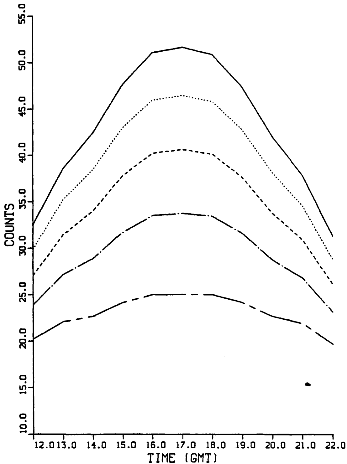
Figure 37. Normalized Cloud Reflectivity as a Function of Video Count and Time of Day for April 16 at 42°N and 74°W, with Calibration Count (C) equal to 60. (Example taken from Huench and Keegan, 1979.)
