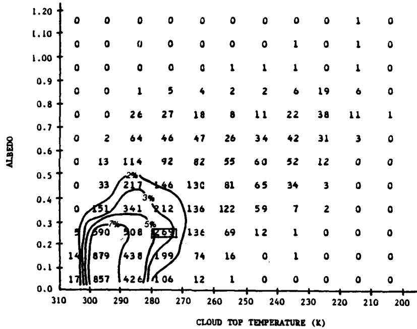
Figure 24. No-Precipitation Overcast and Broken for 10 x 10 Array (The mean, .271 and 279.8K, interval is boxed. The 2%, 3%, 5%, and 7% frequencies are for 147, 221, 368, and 515 occurrences, respectively.)
