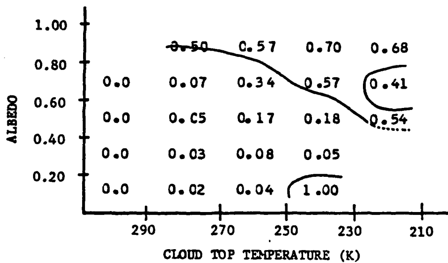
Figure 21. Precipitation Overcast Data Probability 10 x 10 Array Size
