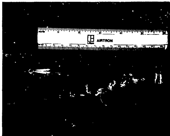
Figure 1. Single crystal boule of Nd:YAG for pilot production run. Boule N3122, photograph taken in ordinary light.
