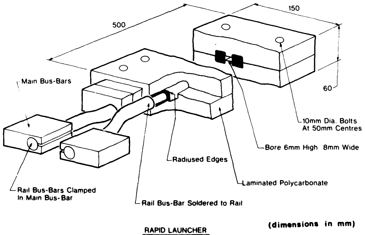
FIGURE 6 isometric drawing showing basic features and dimensions of RAPID
