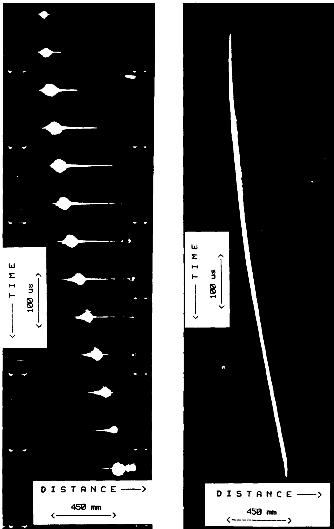
FIGURE 16 Typical framing and streak camera records from a RAPID firing
