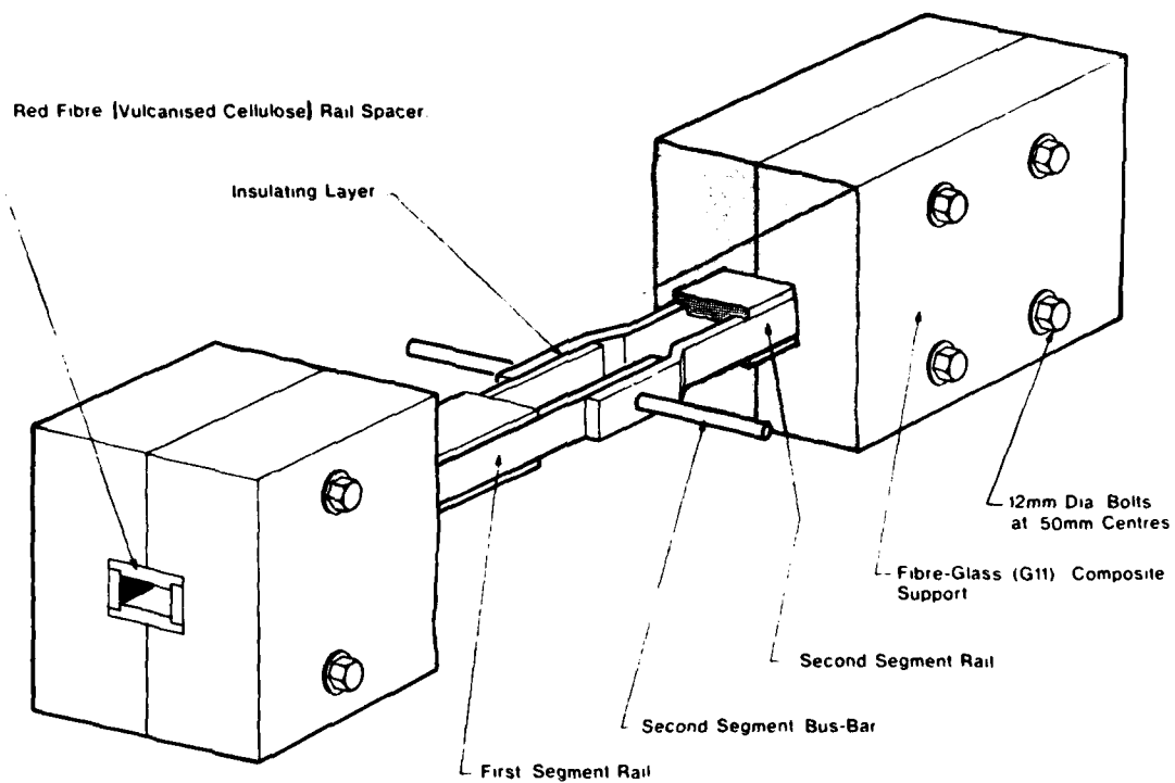
FIGURE 12 Design of segmented railgun (ERGS-3M)
