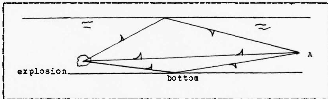
Figure 4.1 Surface Effect on a Shock Wave.
