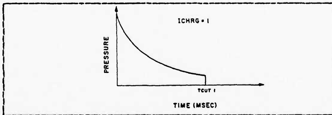
Figure 4.3 Incident Pressure Decay.
