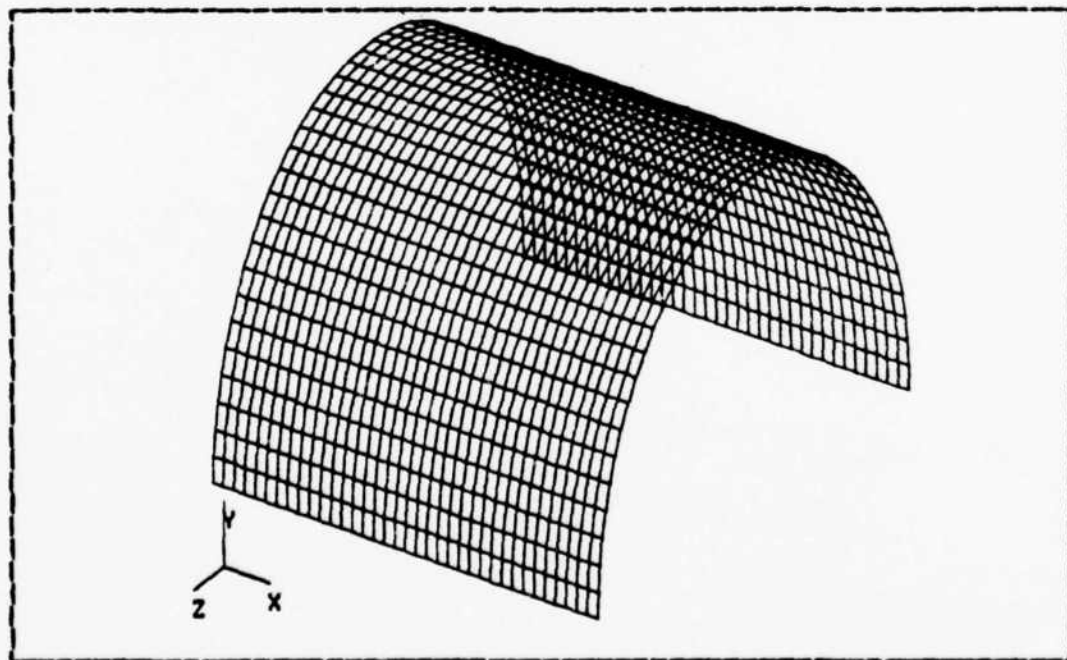
Figure 5.3 FEM Discretization 1517 nodes, 1440 elements.
