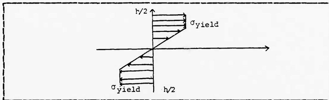
Figure 2.4 Yield Situation in the Shell.
