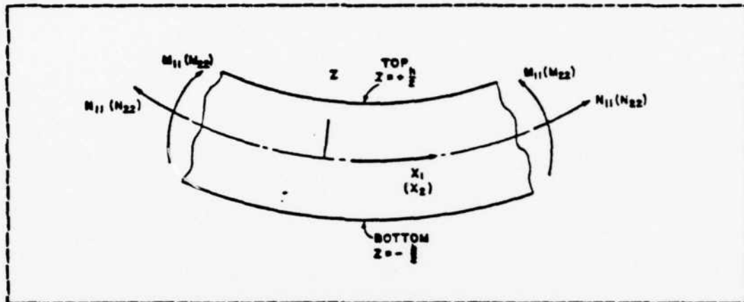
Figure 2.1 Shell Stress State.
