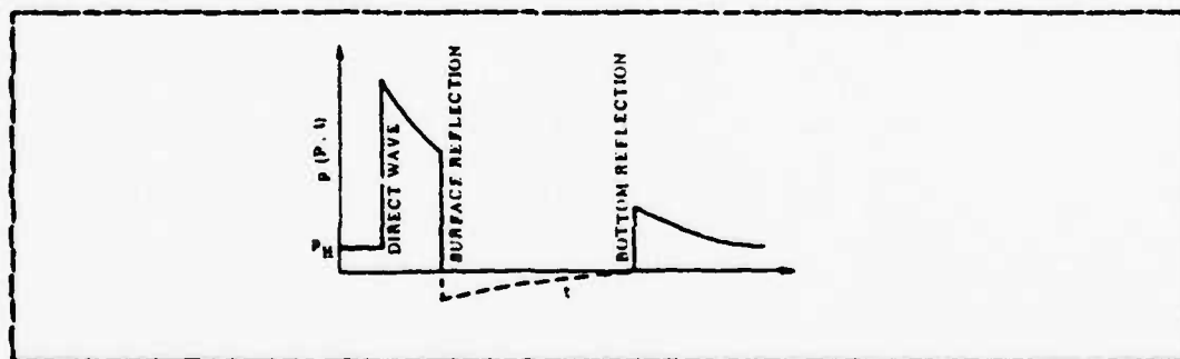
Figure 4.2 Cut-Off Phenomenon.
