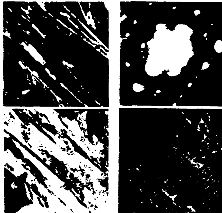
Figure 13. TRANSMISSION ELECTRON MICROGRAPHS OF LASER PROCESSED Fe-0.22C-5Cr ALLOY (PENETRATION DEPTH: 1500 \mu m)
