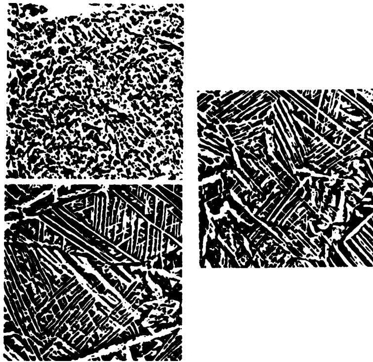
Figure 12. SCANNING ELECTRON MICROGRAPHS SHOWING THE MICROSTRUCTURES OF LASER PROCESSED Fe-0.22C-20Cr ALLOYS a) SINGLE SCAN (PENETRATION DEPTH: 600µm) b) MULTIPLE SCAN (PENETRATION DEPTH: 600µm) c) MULTIPLE SCAN (PENETRATION DEPTH: 120µm) MAGNIFICATION: 1000x.
