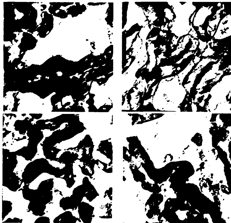
Figure 15. TRANSMISSION ELECTRON MICROGRAPHS OF LASER PROCESSED Fe-0.52C-20Cr ALLOY SHOWING THE AUSTENITE/FERRITE STRUCTURES (PENETRATION DEPTH: 210µm). MAGNIFICATION: 16,000x.
