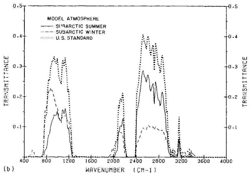
Figure 15. Atmospheric Transmittance for a 10-km Horizontal Path at the surface With the Navy Maritime Aerosol Model. (a) for the tropical, midlatitude summer, and midlatitude winter model atmospheres and (b) for the subarctic summer, subarctic winter, and U.S. Standard atmospheres
