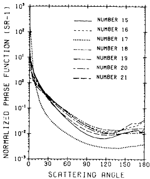
Figure D3. Standard LOWTRAN Phase Functions Numbers 15 to 21
