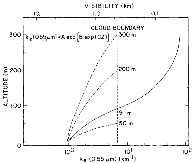
Figure 17. The Vertical Profile of the 0.55- \mu\text{m} Extinction Coefficient for Various Cloud Ceiling Heights. The solid line shows the average profiles from Figure 16, the dashed vertical line represents the value at the cloud boundary
