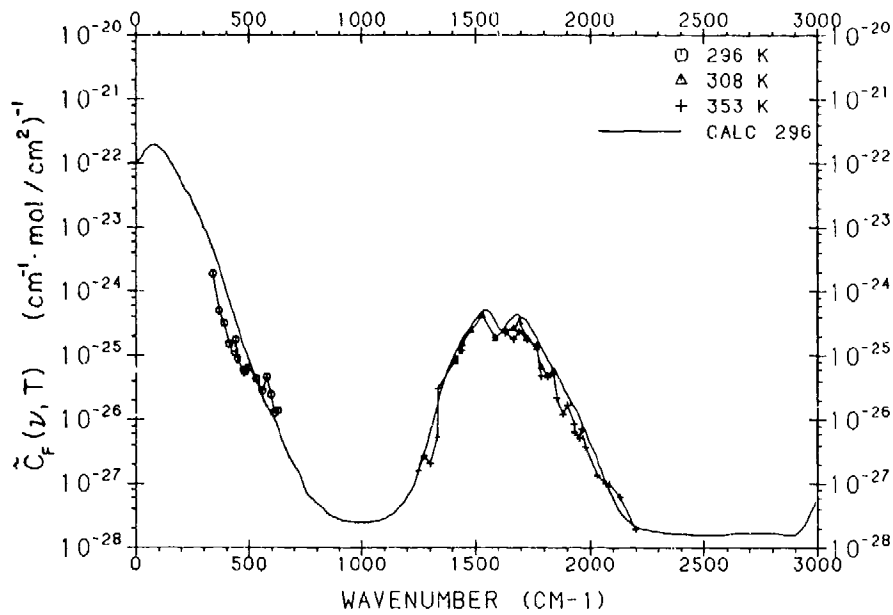
Figure 10. The Foreign Density Dependent Continuum Values, \tilde{C}_f , for Water Vapor as a Function of Wavenumber. The experimental values are from Burch, et al
