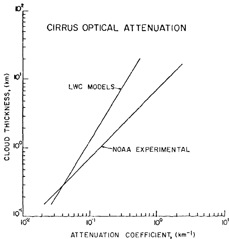
Figure 24. A Comparison of the NOAA Experimental and AFGL Liquid Water Content (LWC) Calculated Attenuation Coefficient for Cirrus. The experimental data curve is chosen for the LOWTRAN model, as explained in the text
