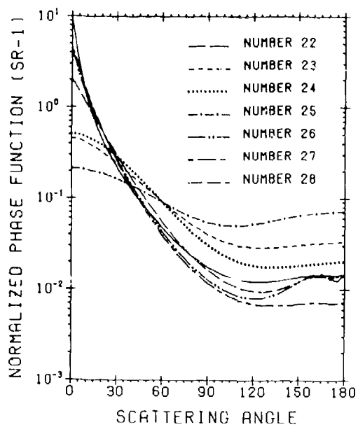
Figure D4. Standard LOWTRAN Phase Functions Numbers 22 to 28
