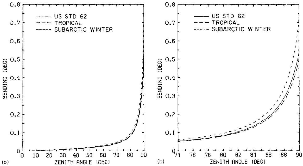
Figure 6. Refractive Bending vs Zenith Angle for Path 1, for Three Atmospheric Profiles. (a) 0 to 90^{\circ} and (b) 74 to 90^{\circ}
