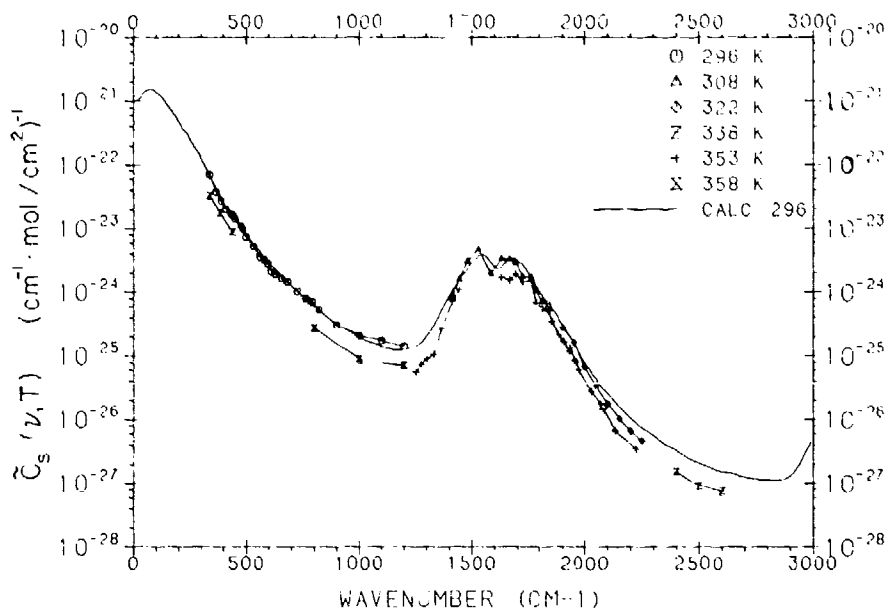
Figure 8. The Self Density Dependent Continuum Values, \hat{C}_s , for Water Vapor as a Function of Wavenumber. The experimental values are from Burch, et al
