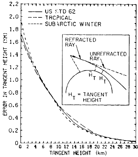
Figure 5. Unrefracted Tangent Height Minus Refracted Tangent Height vs Refracted Tangent Height for a Ray Coming in From Space for Three Atmospheric Profiles. The figure in the inset illustrates the paths
