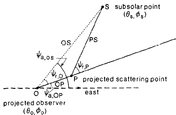
Figure C1. Looking Down on the Scattering Path. All points are projected on the earth and all line segments are parts of great circles. The relative azimuth can be seen to vary as one moves the scattering point along OP
