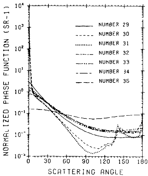
Figure D5. Standard LOWTRAN Phase Functions Numbers 29 to 35
