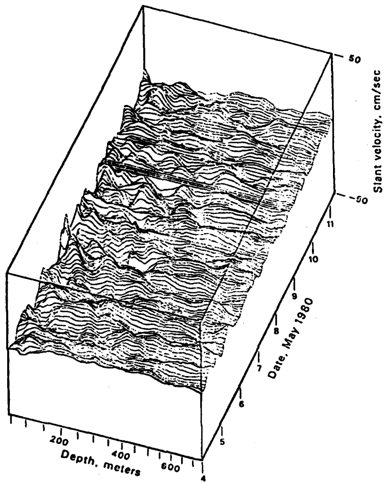
70 kHz VELOCITY PROFILE 7 DAY RECORD
