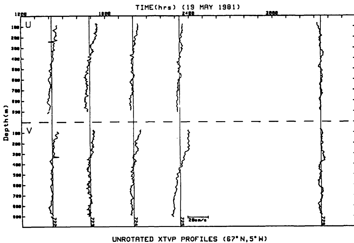
FIGURE 3. XCP (XTVP) DATA COLLECTED IN MAY 1981.
