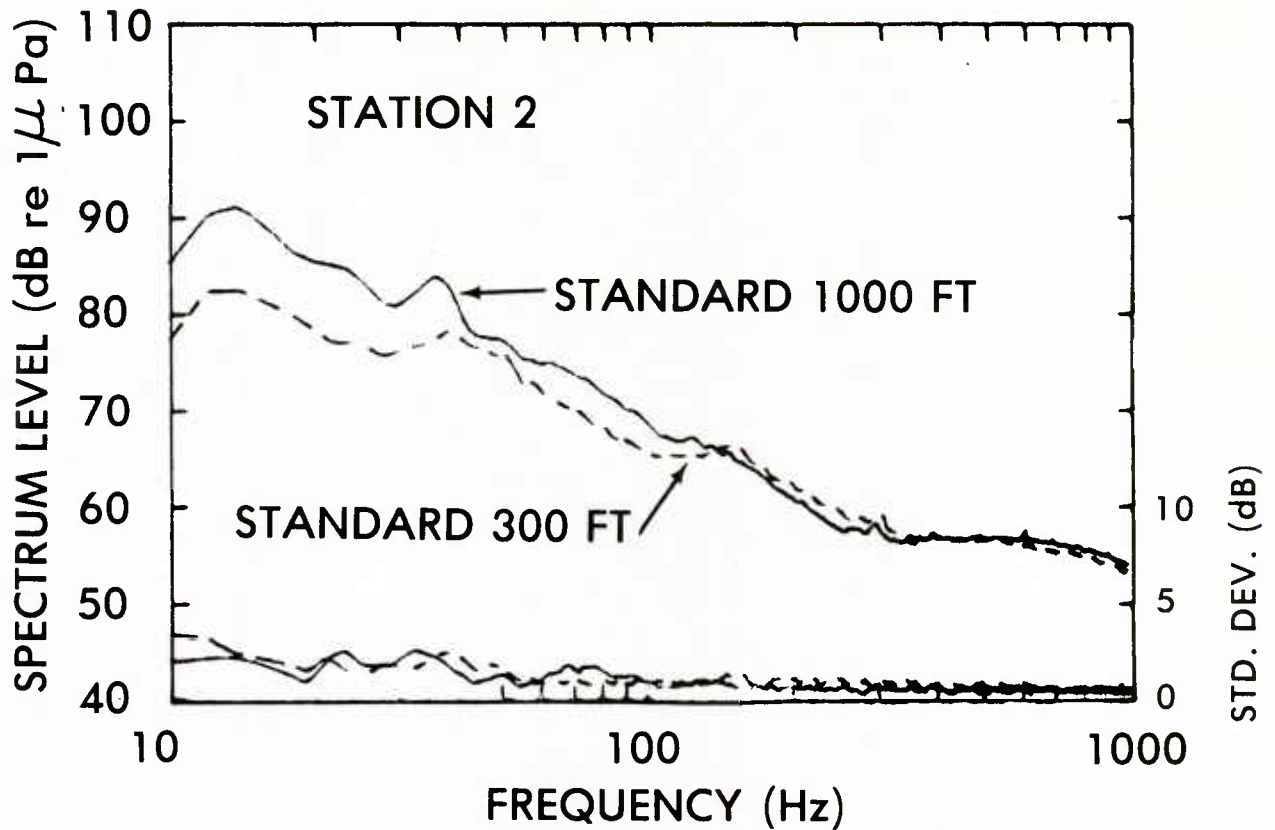
Figure 4B. Ambient noise spectral values from standard sonobuoys at Station 2. Upper curves for each acoustic station represent the 2-Hz ambient noise levels from standard SSQ-57A (300 ft) and standard SSQ-57A (XN-5) (1000 ft) sonobuoys. The lower curves represent the respective standard deviations (scale shown at right). Solid line, 1000 ft; dashed line, 300 ft. The increased values of noise of the 1000 ft buoys below 100 Hz are due to increased self-noise of the measuring system.
