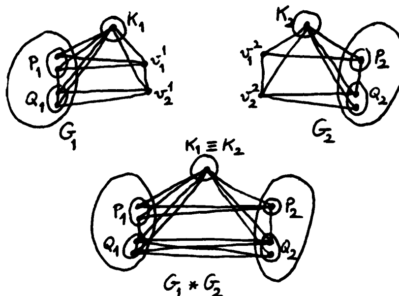
Figure 1. An example of the 2-amalgam composition.
