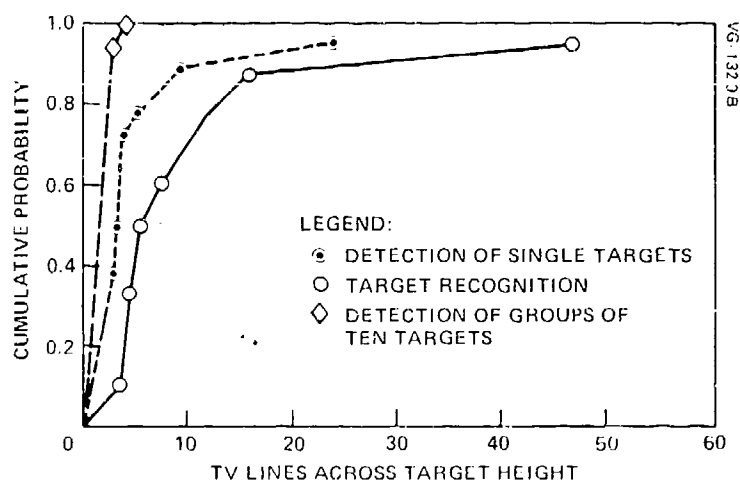
Figure 28. Target detection and recognition line criteria.
