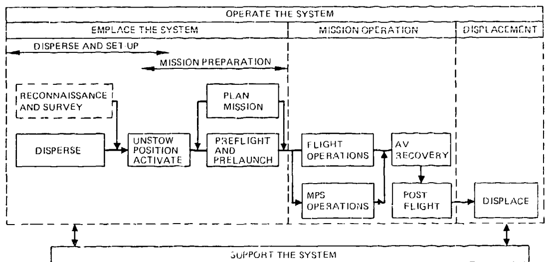
Figure 39. Top level RPV system operations.
