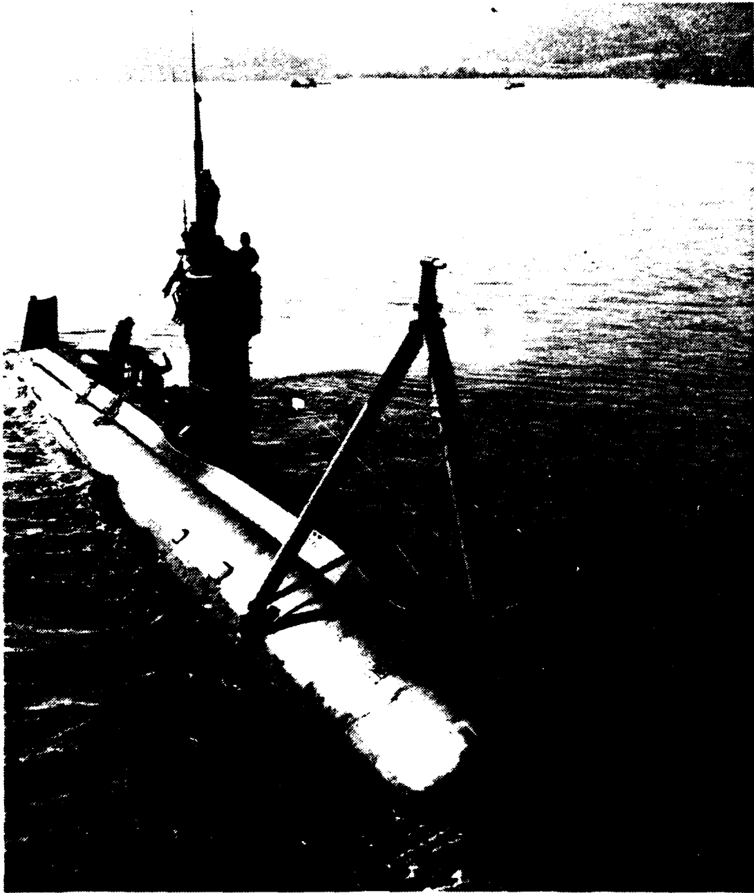
Figure 1. Photograph of Instruments. The turbulence package was mounted on top the tripod 4.2m above the deck of the USF DOLPHIN. The NBIC STD transducers and one acoustic current meter were located 0.5m below the turbulent package.
