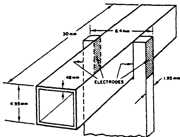
Figure 4. Schematic Illustration of Conductivity Sensor. Schematic illustration of the geometry of the conductivity sensor, which is the standard for use with NBIS CTD system. Two of the four electrodes are shown and could be either the current or voltage pair. (From Gregg & Schedvin, "Dynamic Response Calibration of the Neil Brown Conductivity Cell", Journal of Physical Oceanography , Vol. 12, 1982)
