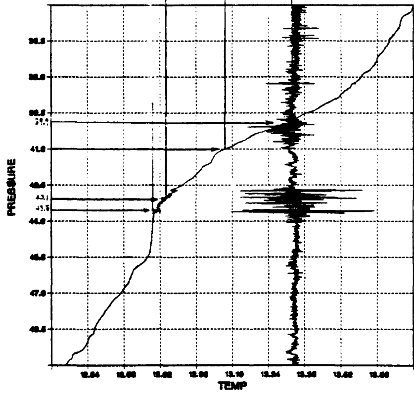
Figure 15. The CTD Data for the Two Different Signatures Shown in Figure 3. The upper patch (salt fingers (S.F.)) shows the value of R less than 2 in upper portion, and about 2 in lower portion. The thickness of the upper patch is almost the same as in Figure 3, but the lower patch is different from the one in Figure 3 due to the spatial variations of the turbulent patch (T.P.)
