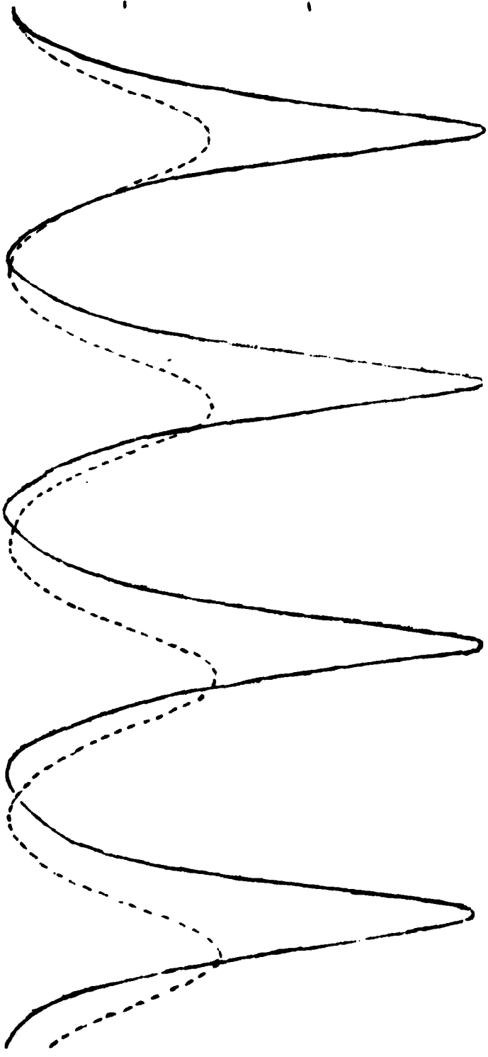
Figure 7: The wave envelope |y(t, x)| p=2+0.1x , a=0 , b=0.1x
