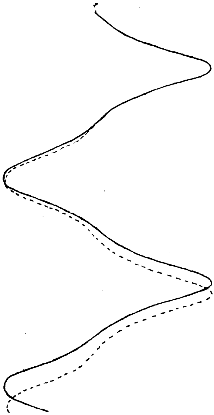
Figure 5: The wave envelope |\psi(0,x)| P=2+0.1X , \alpha = \pi/2 , \beta = 0.1 .
