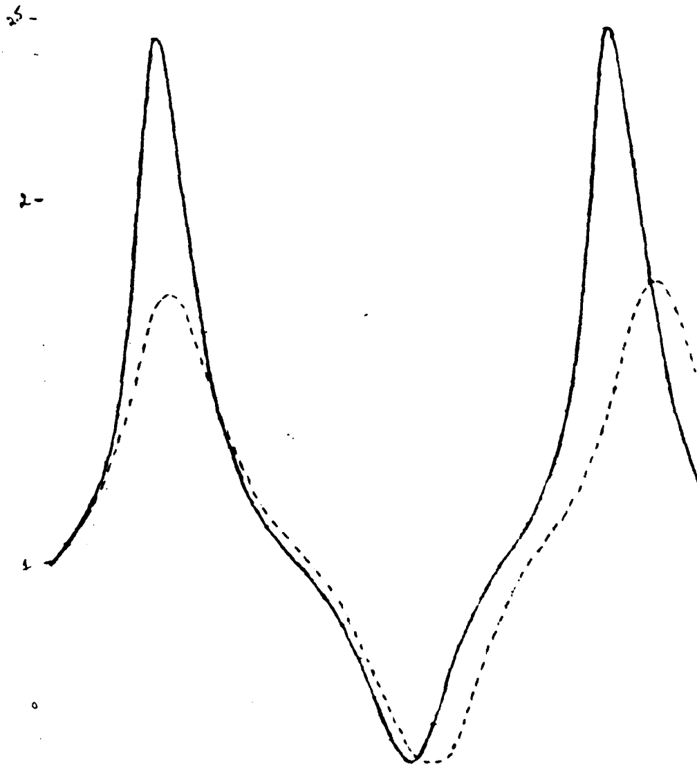
Figure 9: The wave envelope |\psi(0,x)|
