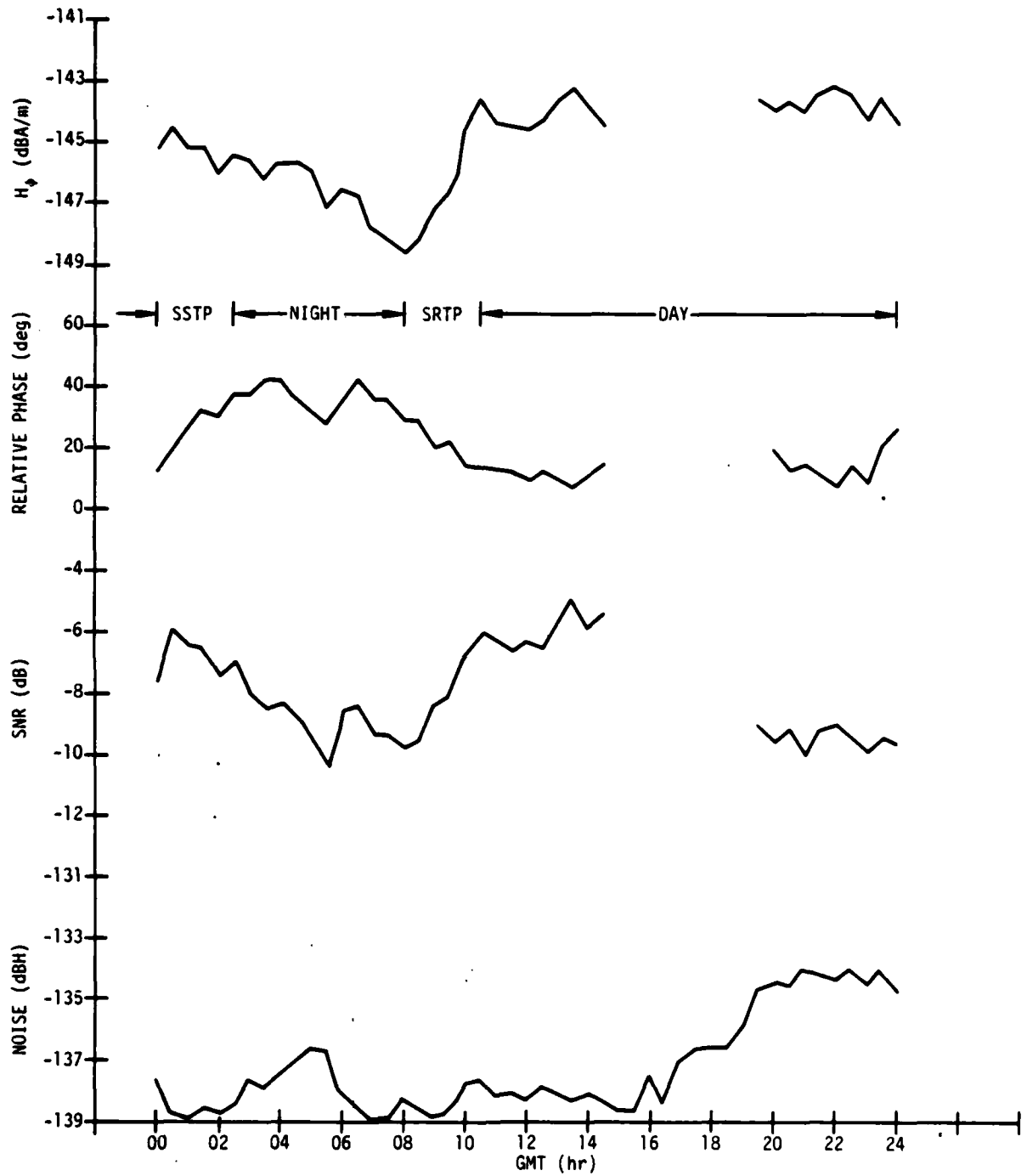
Figure A-8 Connecticut Data Versus GMT ( \psi = 291 deg), 9 May 1977
