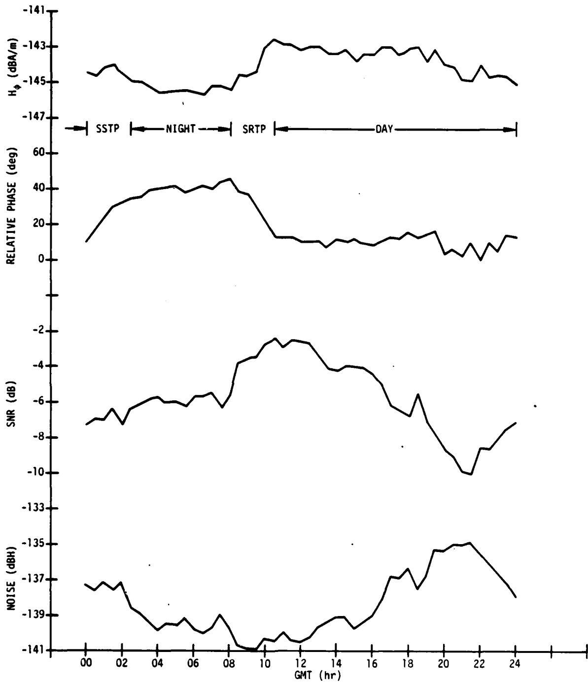
Figure A-6. Connecticut Data Versus GMT (\psi = 291 \text{ deg}) , 7 May 1977
