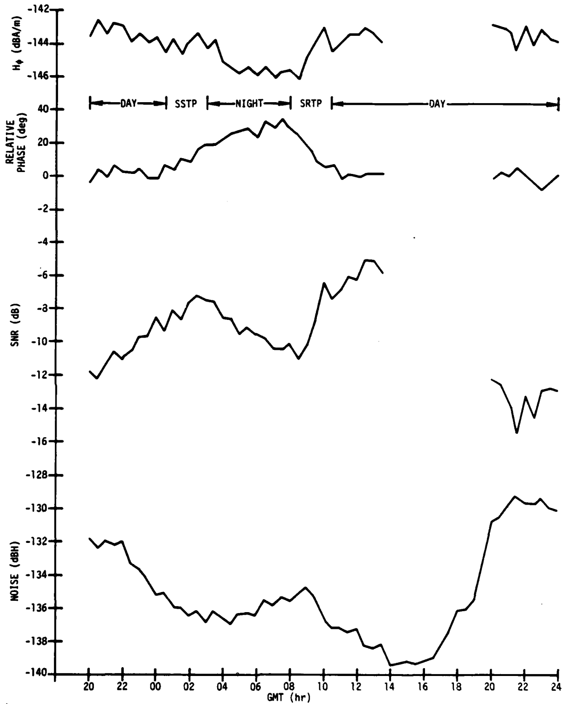
Figure B-16. Connecticut Data Versus GMT ( \psi = 291 deg), 20 June 1977
