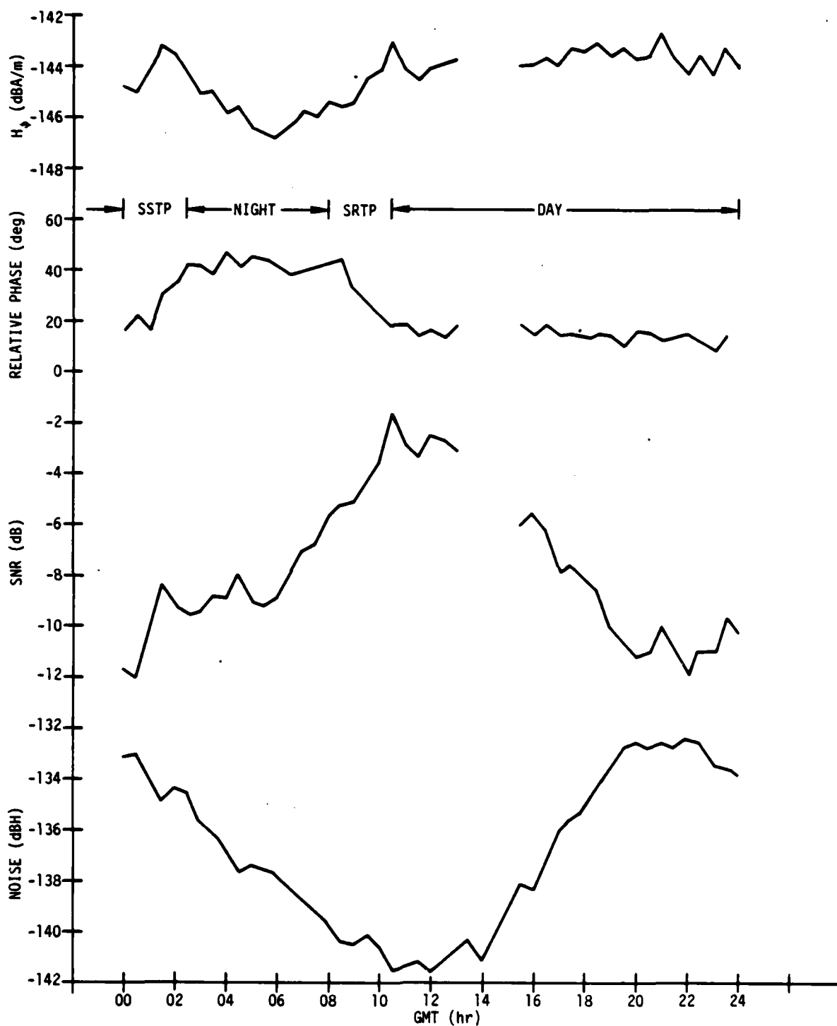
Figure A-18. Connecticut Data Versus GMT ( \psi = 291 deg), 20 May 1977
