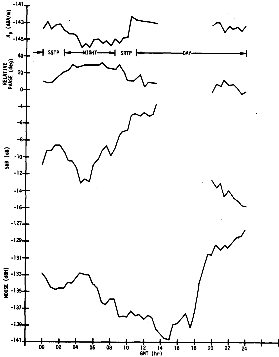
Figure C-14. Connecticut Data Versus GMT ( \psi = 291 deg), 24 July 1977
