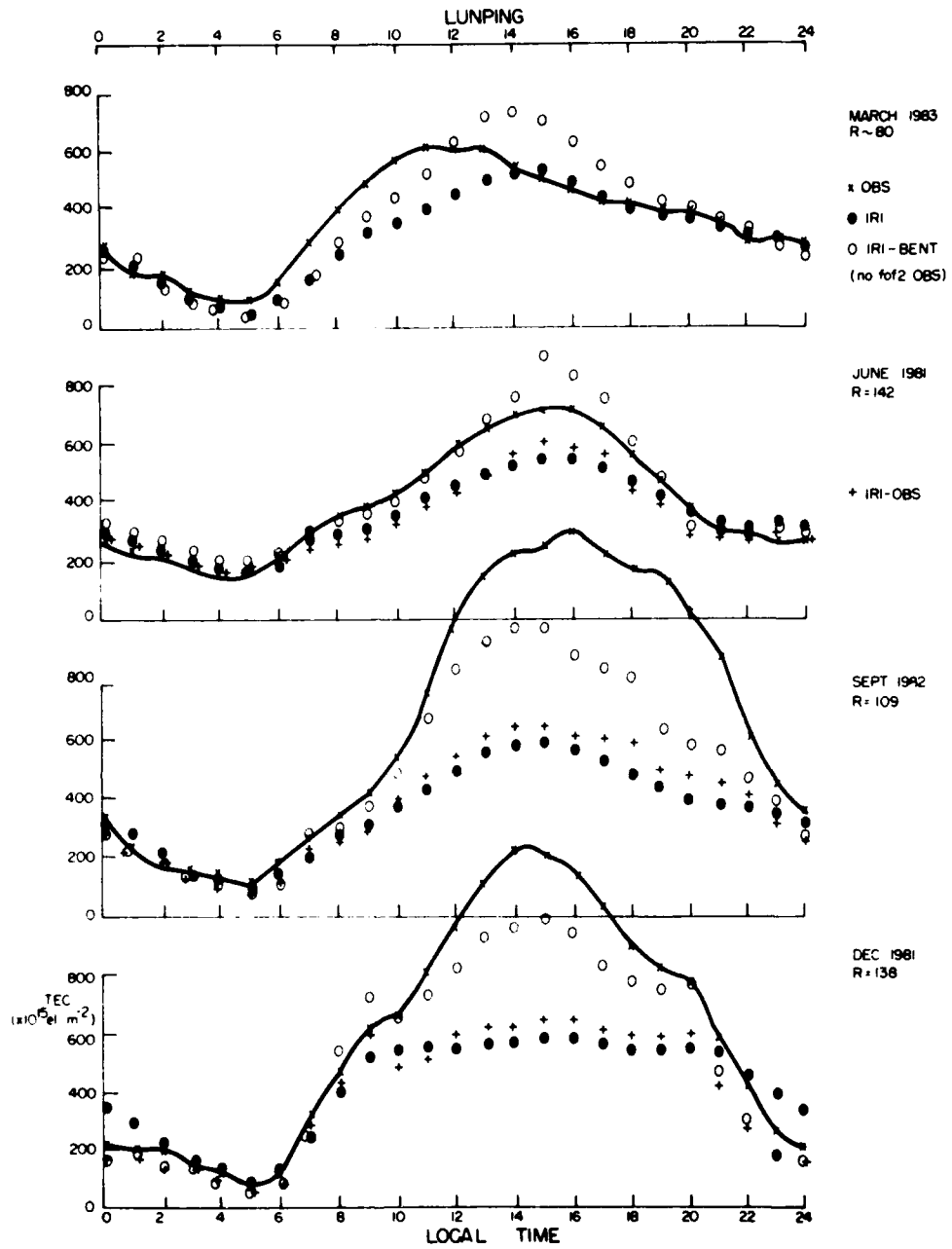
Figure 10. Predicted and Observed Values of TEC at Lunping (Taiwan) for Four Months With High Solar Activity (1981, 1982, 1983)
