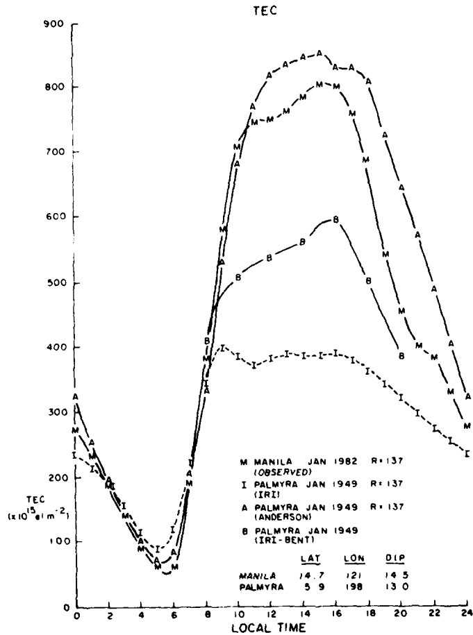
Figure 21. Calculated and Observed Values of TEC for January at a Station at 13^\circ Dip, for R = 137 . The observed values are for Manila, while calculated values are given for the IRI, the modified IRI-BENT and the Anderson theoretical models. The Anderson values were calculated for Palmyra
