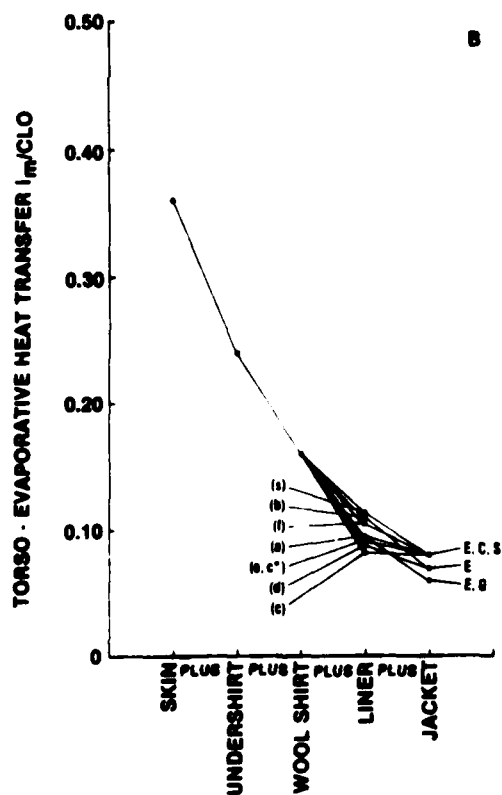
Figure 6. Evaporative heat transfer coefficient ( i_m/clo ) plotted against the clothing components on the: A. Arms, B. Torso, and C. Torso and Arms
