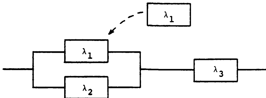
Figure 3. Combined Serial/Parallel System with Spare
