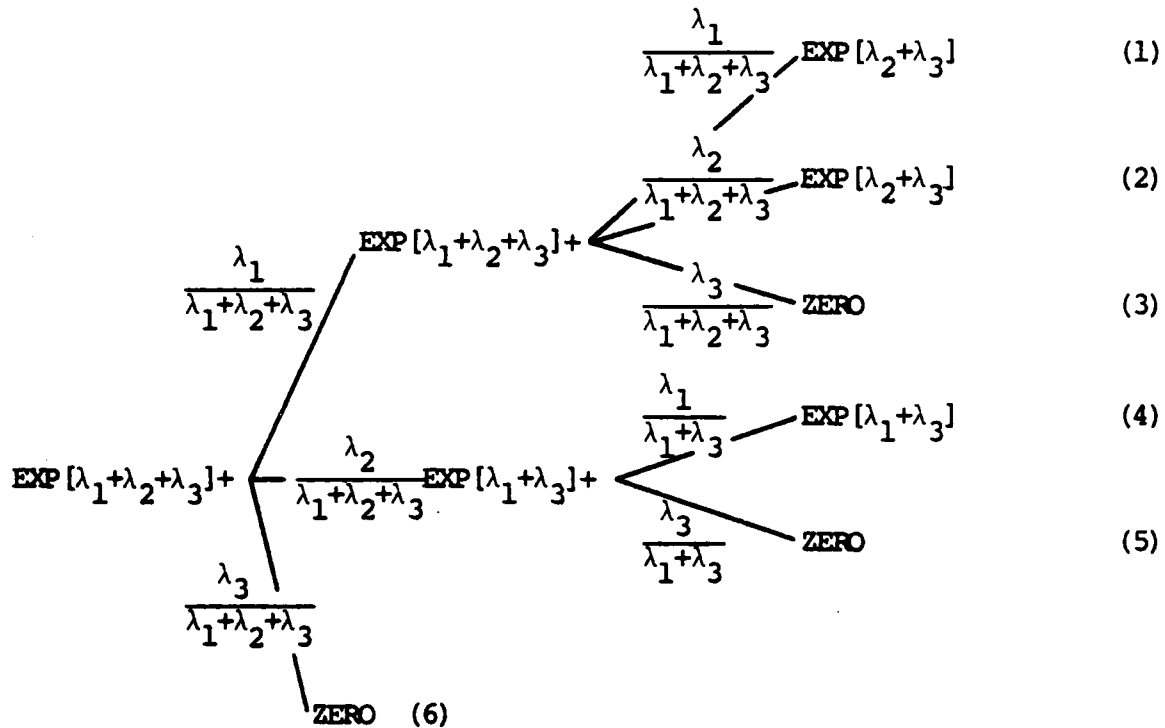
Figure 4. Shorthand Branching Diagram for Serial/Parallel System with Spare
