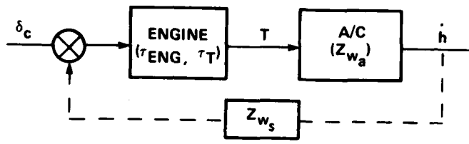
Fig. 1. VTOL vertical control: Fixed wing (jet lift).
