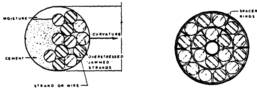
a. Improper grouting and spacing b. Wires with proper spacing
